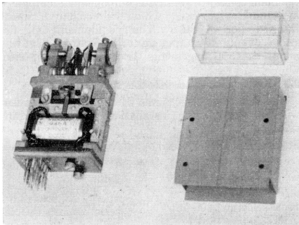
FIG. 13.—CARPENTER RELAY.
