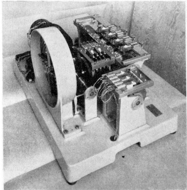
FIG. 15.—SIGNAL GENERATOR.
