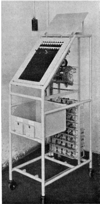
FIG. 25.—TESTER FOR TRUNK RELAY SET.
