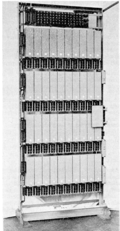
FIG. 14.—FINAL SELECTOR RACK.
