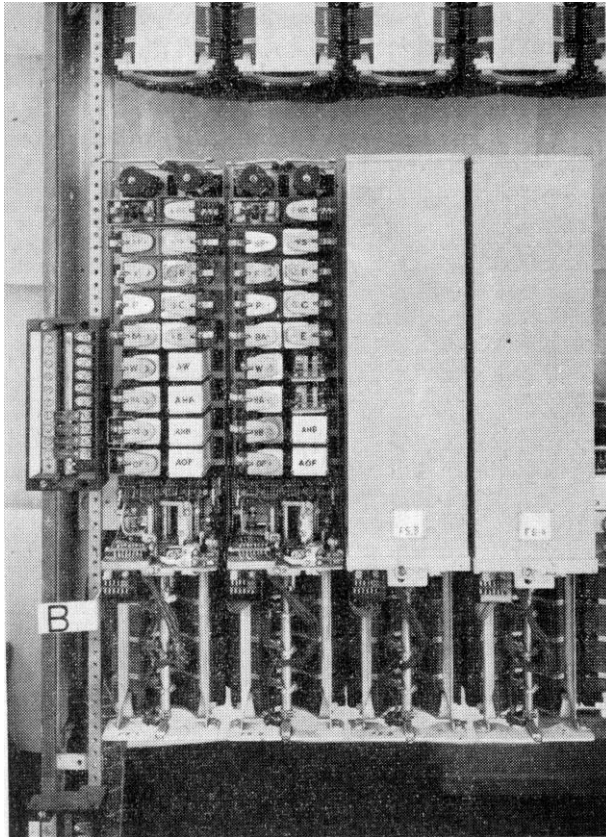
FIG. 12. FINAL SELECTOR.
