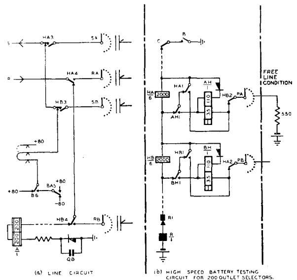
FIG. 21.—GROUP SELECTOR ELEMENTS.
