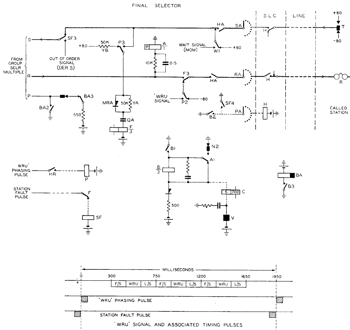
FIG. 22.—FINAL SELECTOR LINE, IMPULSING AND CALLING ELEMENTS.
