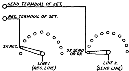
FIG.5. 2 LINE SIMPLEX CIRCUIT.
