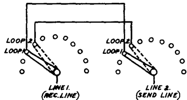
FIG 7. 2 LINES LOOPED.
