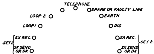
FIG. 2. NORMAL LABELLING OF SWITCH. (LABEL No. 284B BLACK)
