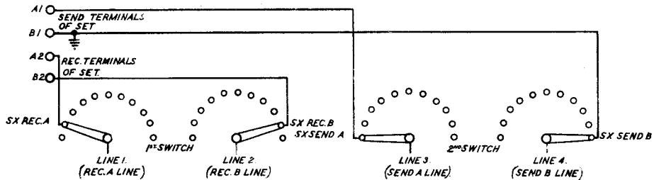
FIG 8. 2 LOOP SIMPLEX CIRCUIT
