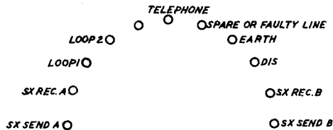
FIG. 3. LABELLING OF SWITCH FOR 2 LOOP SIMPLEX TERMINATIONS ONLY. (LABEL No. 284A BLACK)
