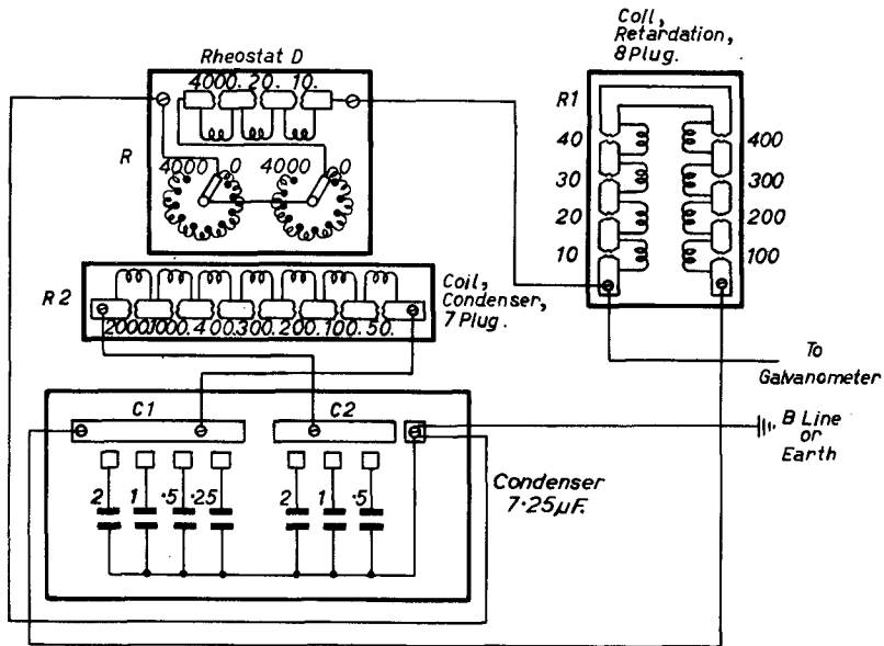
WIRING CONNECTIONS.
