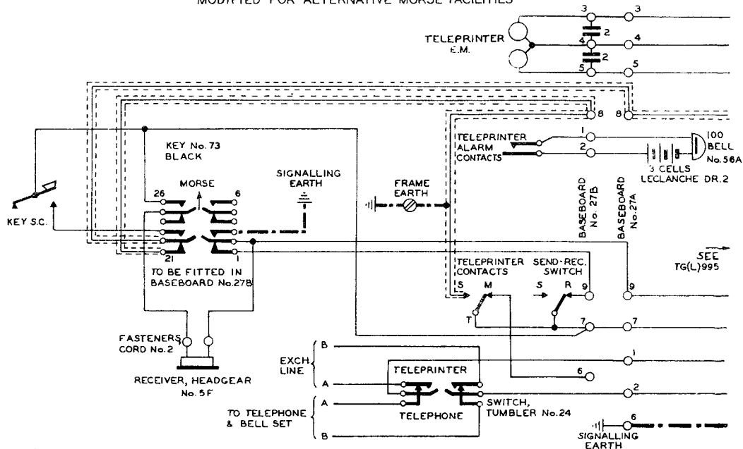
FIG. 2. USING TELETYPE WITHOUT SEND-RECEIVE SWITCH LOCAL RECORD.
