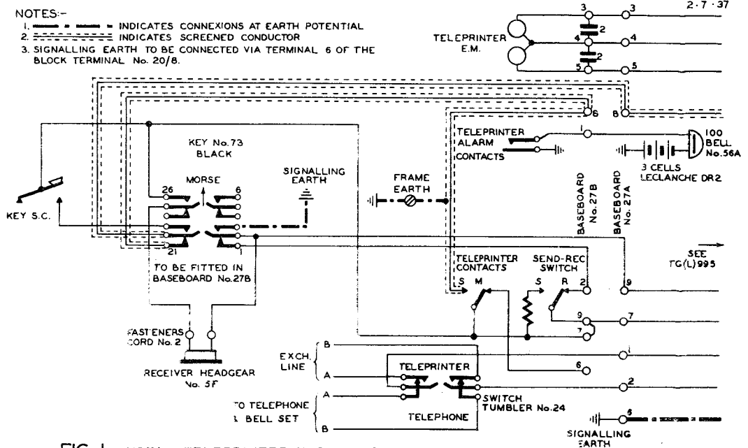
FIG. 1 USING TELETYPE WIRED FOR SEND-RECEIVE SWITCH LOCAL RECORD
