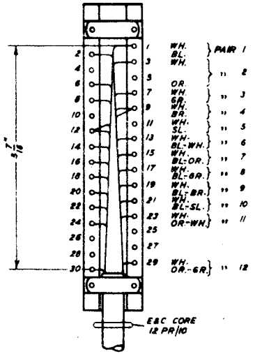
EXTERNAL EXTENSION UNIT STRIP
