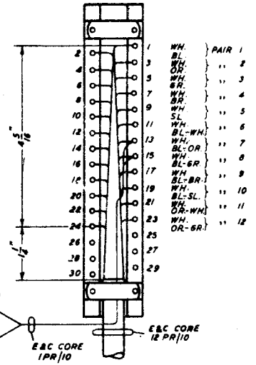
MAIN JUNCTION BOX STRIP
