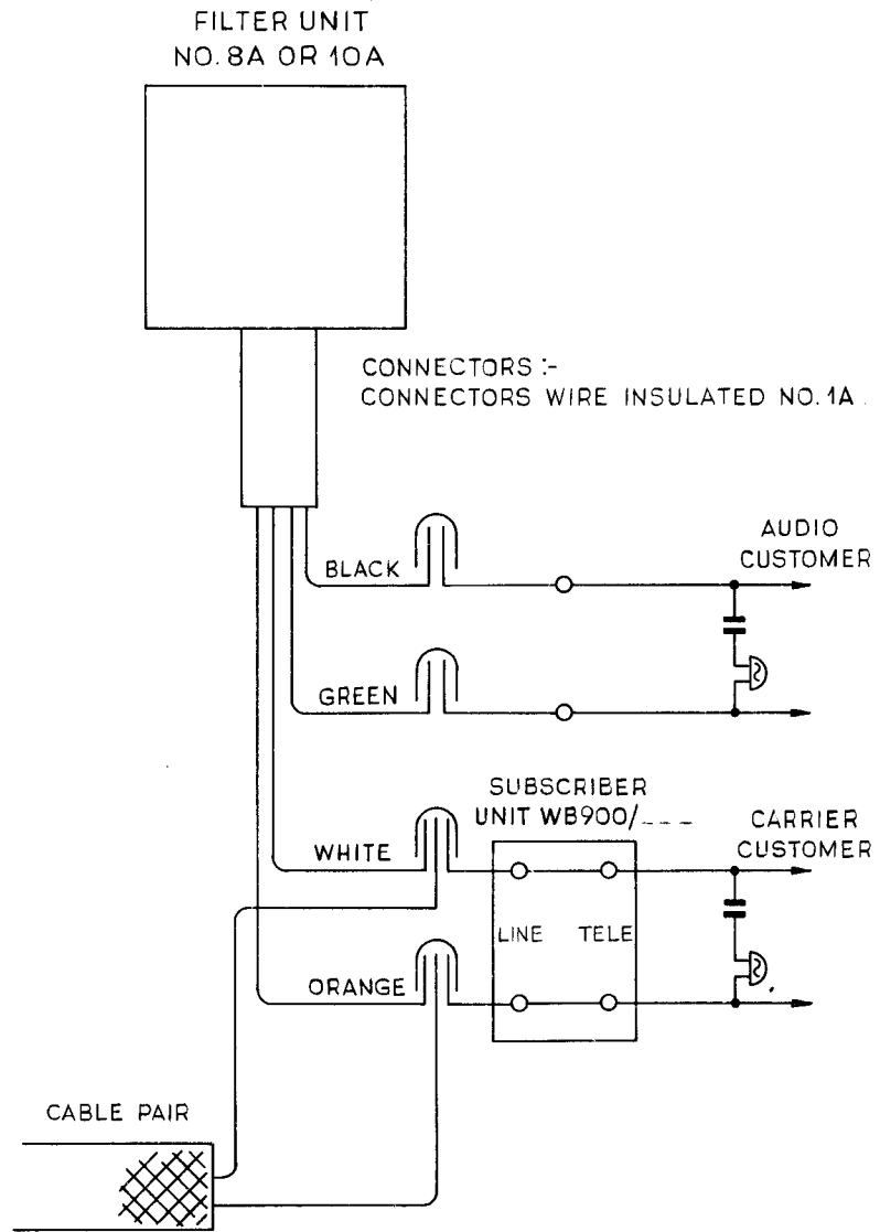
RECOMMENDED METHOD OF CONNECTING FILTERS UNDERGROUND CONSTRUCTION
