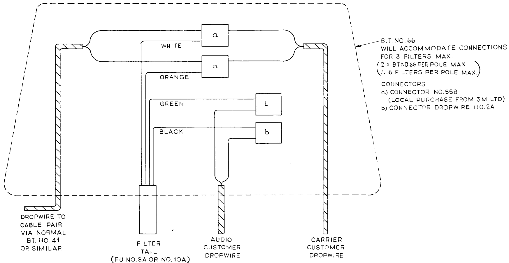
RECOMMENDED METHOD FOR WB 900 FILTER CONNECTIONS (OVERHEAD CONSTRUCTION)
