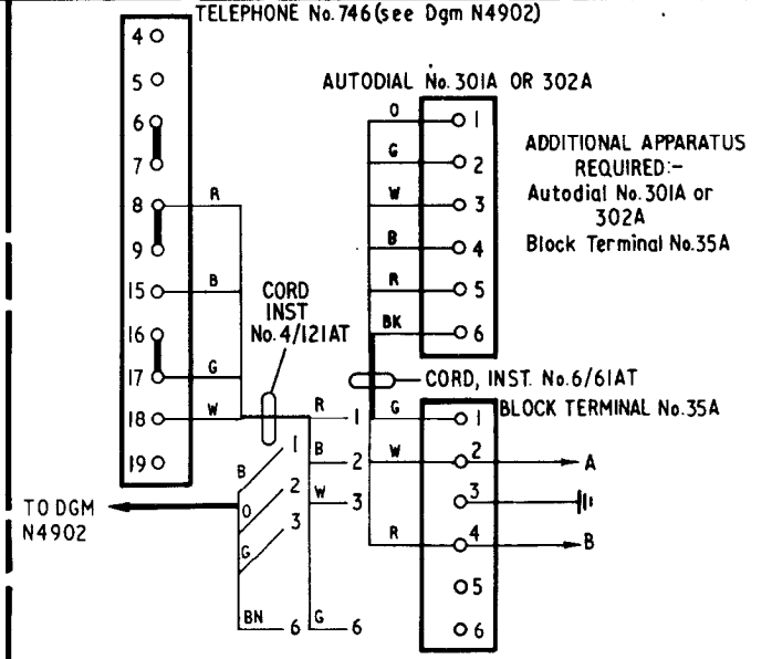
FIG. 13 USING TELEPHONE No. 746 SHARED SERVICE (SEPARATE METERING) Connexions as shown EXCLUSIVE SERVICE Earth and green cable connexions to BT3 omitted. T4-T5, T18-T19 and BT2-BT3 strapped.
