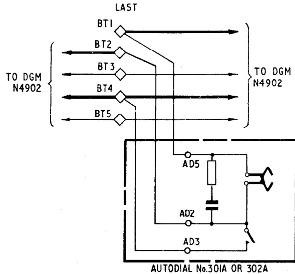
FIG. 2 USING TELEPHONE SR I... B SHARED SERVICE (SEPARATE METERING) Connexions as shown. EXCLUSIVE SERVICE Connexions to BT5 omitted.
