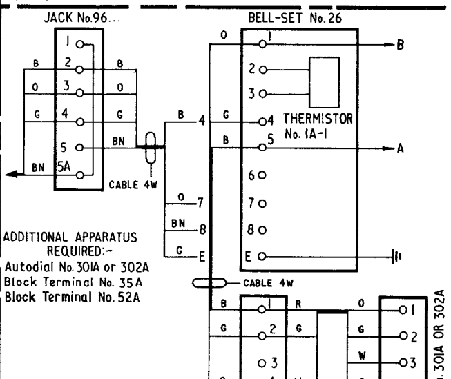
FIG. 19 SHARED SERVICE (SEPARATE METERING) Connections as shown EXCLUSIVE SERVICE Earth and green cable connexions to J4 and E omitted. J3 and J4 strapped. Thermistor No. 1A-1 omitted. B2-B3 strapped.
