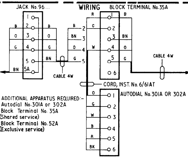
FIG. 18 SHARED SERVICE (SEPARATE METERING) Connections as shown EXCLUSIVE SERVICE Green cable connexions to BT5 and J4 omitted. J3 and J4 strapped.
