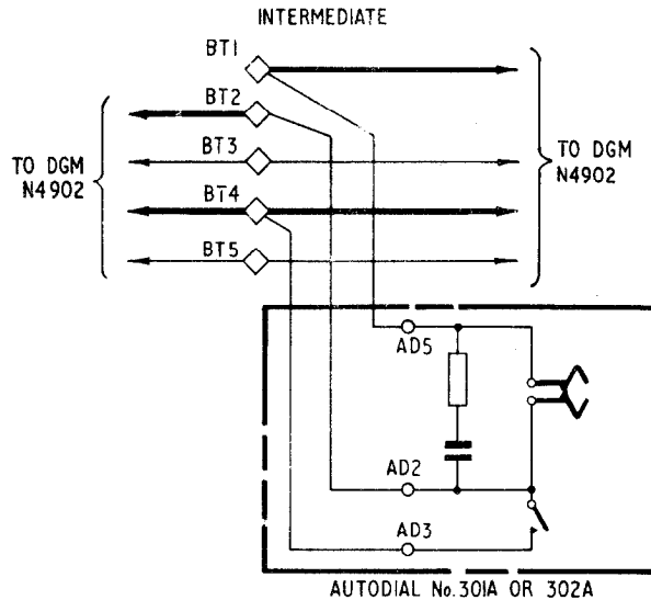
FIG. 3 USING TELEPHONE SR I... B SHARED SERVICE (SEPARATE METERING) Connexions as shown. EXCLUSIVE SERVICE Connexions to BT5 omitted
