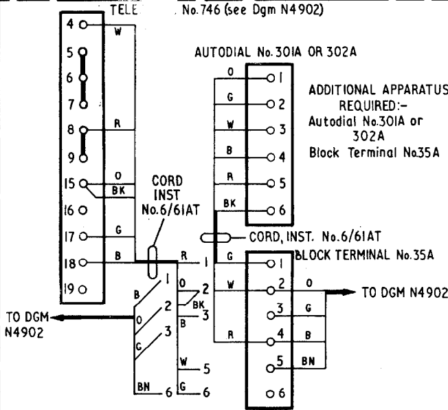
FIG. 12 USING TELEPHONE No. 746 SHARED SERVICE (SEPARATE METERING) Connexions as shown EXCLUSIVE SERVICE Green cable connexions to BT3 omitted. Cord, Inst. No. 4/121AT used in lieu, omitting orange and black connexions to BT2 and T15. T18-T19 and BT2-BT3 strapped.
