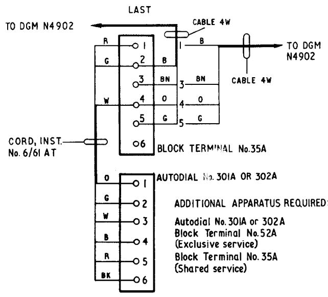
FIG. 8 USING TELEPHONE SRI...B SHARED SERVICE (SEPARATE METERING) Connexions as shown. EXCLUSIVE SERVICE Green cable connexionsto BT5 omitted.
