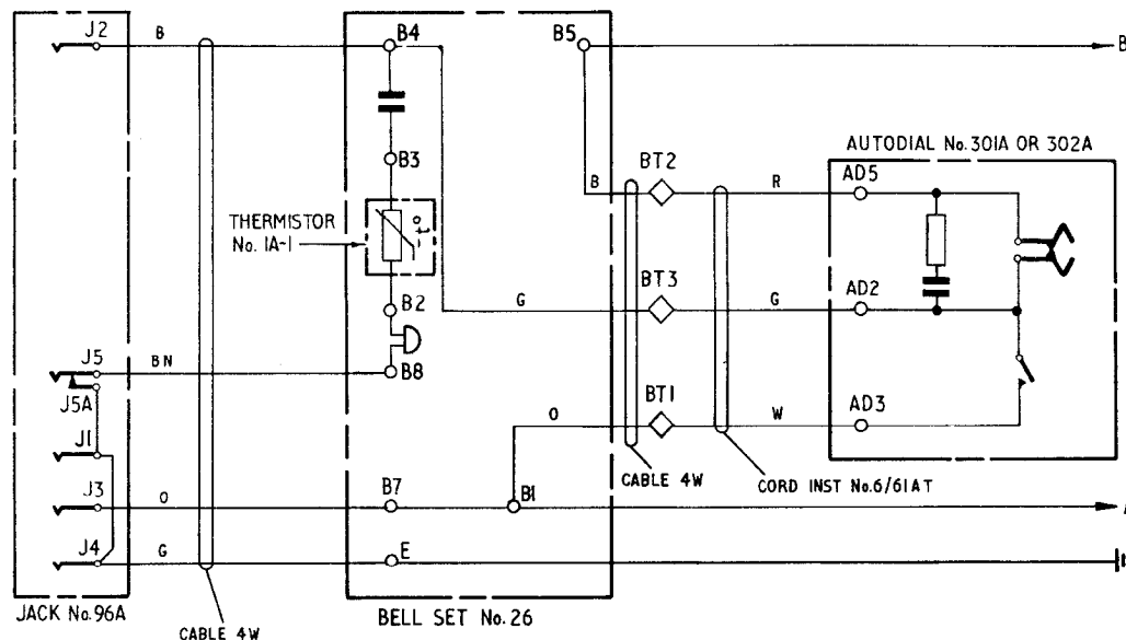
FIG. 1 AUTODIAL No. 301A OR 302A CONNECTED TO A DIRECT EXCHANGE LINE
