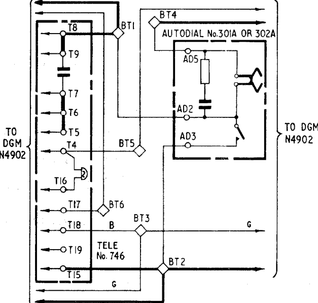
FIG. 6 USING TELEPHONE No. 746 SHARED SERVICE (SEPARATE METERING) Connexions as shown. EXCLUSIVE SERVICE Green cable connexions to BT3 omitted. T18-T19 and BT2-BT3 strapped.
