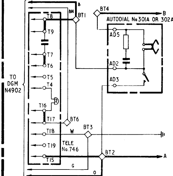
FIG. 7 USING TELEPHONE No. 746 SHARED SERVICE (SEPARATE METERING) Connexions as shown. EXCLUSIVE SERVICE Earth and green cable connexions to BT3 omitted. T4-T5, T18-T19 and BT2-BT3 strapped.
