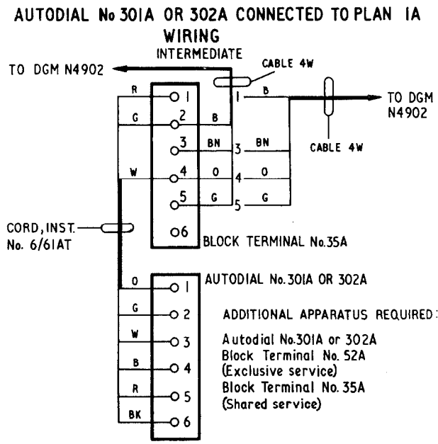
FIG. 9 USING TELEPHONE SRI...B SHARED SERVICE (SEPARATE METERING) Connexions as shown. EXCLUSIVE SERVICE Green cable connexionsto BT5 omitted.
