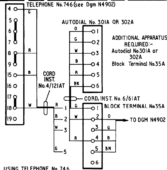
FIG. 11 USING TELEPHONE No. 746 SHARED SERVICE (SEPARATE METERING) Connexions as shown EXCLUSIVE SERVICE Green cable connexion to BT3 omitted. Strap T17-T18 omitted, T18-T19 and BT2-BT3 strapped. Shift blue cord conductor from T15 to T17
