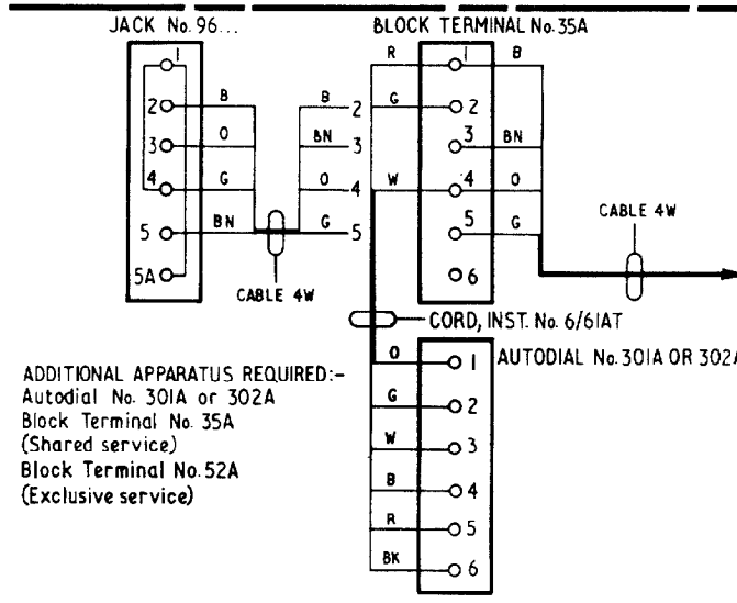
FIG. 17 SHARED SERVICE (SEPARATE METERING) Connections as shown EXCLUSIVE SERVICE Green cable connexions to BT5 and J4 omitted. J3 and J4 strapped.
