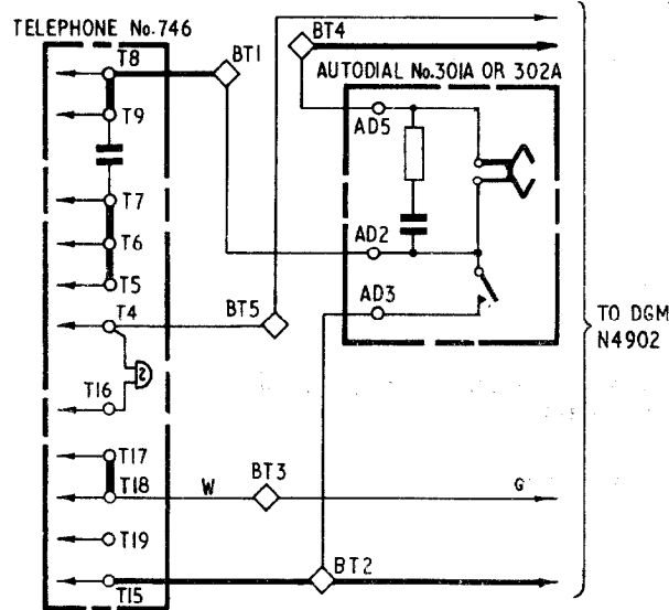
FIG. 5 USING TELEPHONE No. 746 SHARED SERVICE (SEPARATE METERING) Connexions as shown. EXCLUSIVE SERVICE Green cable connexion to BT3 omitted. Strap T17-T18 omitted. T18-T19 and BT2-BT3 strapped. BT2 connected to T17 instead of to T15.
