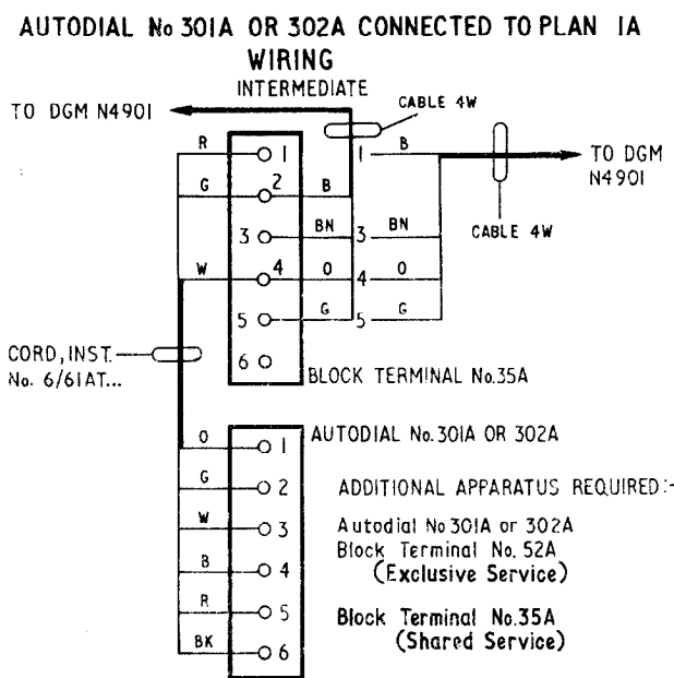
FIG. 9 USING TELEPHONE SRI...A SHARED SERVICE (SEPARATE METERING) Connexions as shown. EXCLUSIVE SERVICE Green cable connexions to BT5 omitted
