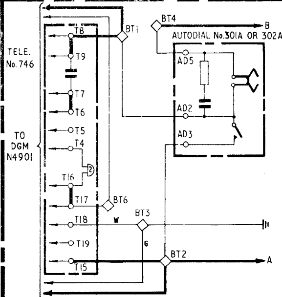
FIG. 7 USING TELEPHONE No. 746
