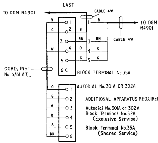
FIG. 8 USING TELEPHONE SRI...A SHARED SERVICE (SEPARATE METERING) Connexions as shown. EXCLUSIVE SERVICE Green cable connexions to BT5 omitted
