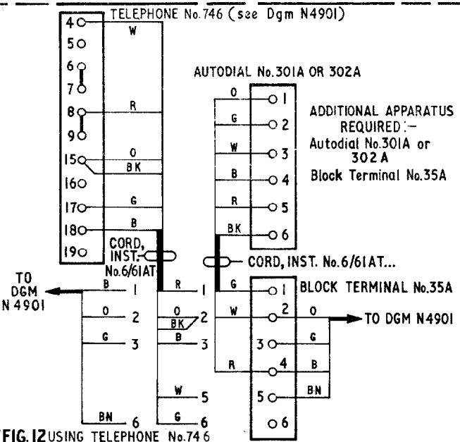
FIG. 12 USING TELEPHONE No. 746 SHARED SERVICE (SEPARATE METERING) Connexions as shown EXCLUSIVE SERVICE Green cable connexions to BT3 omitted. Cord, Inst. No. 4/121 AT used in lieu of omitting orange and black connexions to BT2 and T15. T18-T19 and BT2-BT3 strapped.
