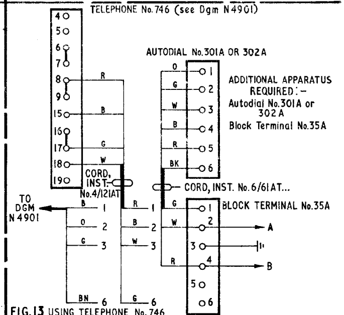
FIG. 13 USING TELEPHONE No. 746 SHARED SERVICE (SEPARATE METERING) Connexions as shown EXCLUSIVE SERVICE Earth and green cable connexions to BT3 omitted. T4-T5, T18-T19 and BT2-BT3 strapped.
