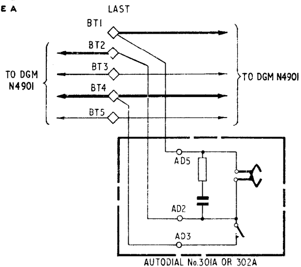
FIG. 2 USING TELEPHONE SR 1...A
