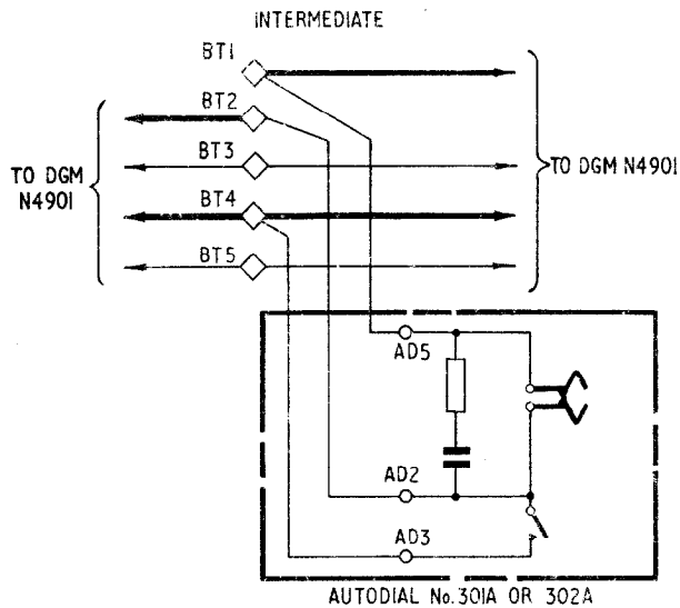
FIG. 3 USING TELEPHONE SR 1...A
