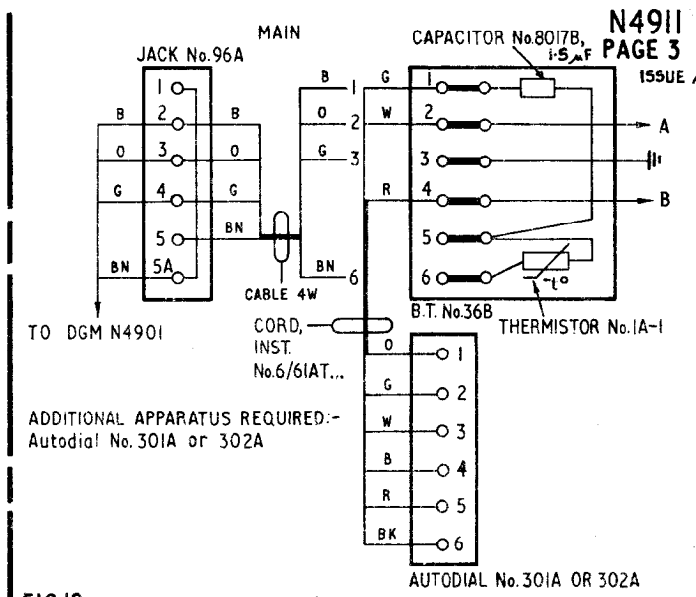
FIG. 10 USING TELEPHONE SRI...A SHARED SERVICE (SEPARATE METERING) Connexions as shown. EXCLUSIVE SERVICE Earth and green cable connexions to BT3, J4 omitted. J3-J4 strapped. Thermistor No. IA-1 omitted, BT5-BT6 strapped.
