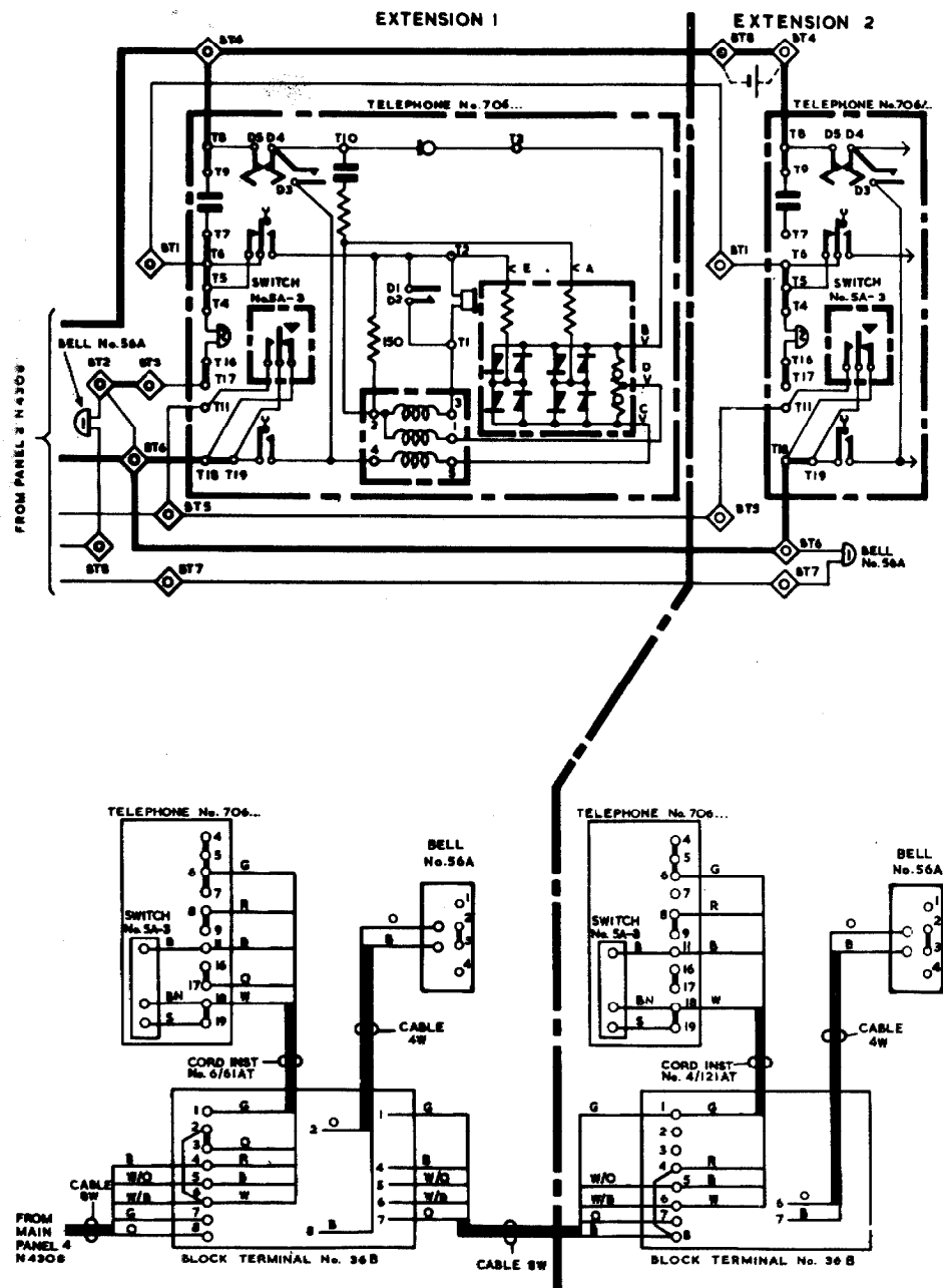
FIG. 1. EXTENSIONS FROM BELL SET No. 39A OR 44.
