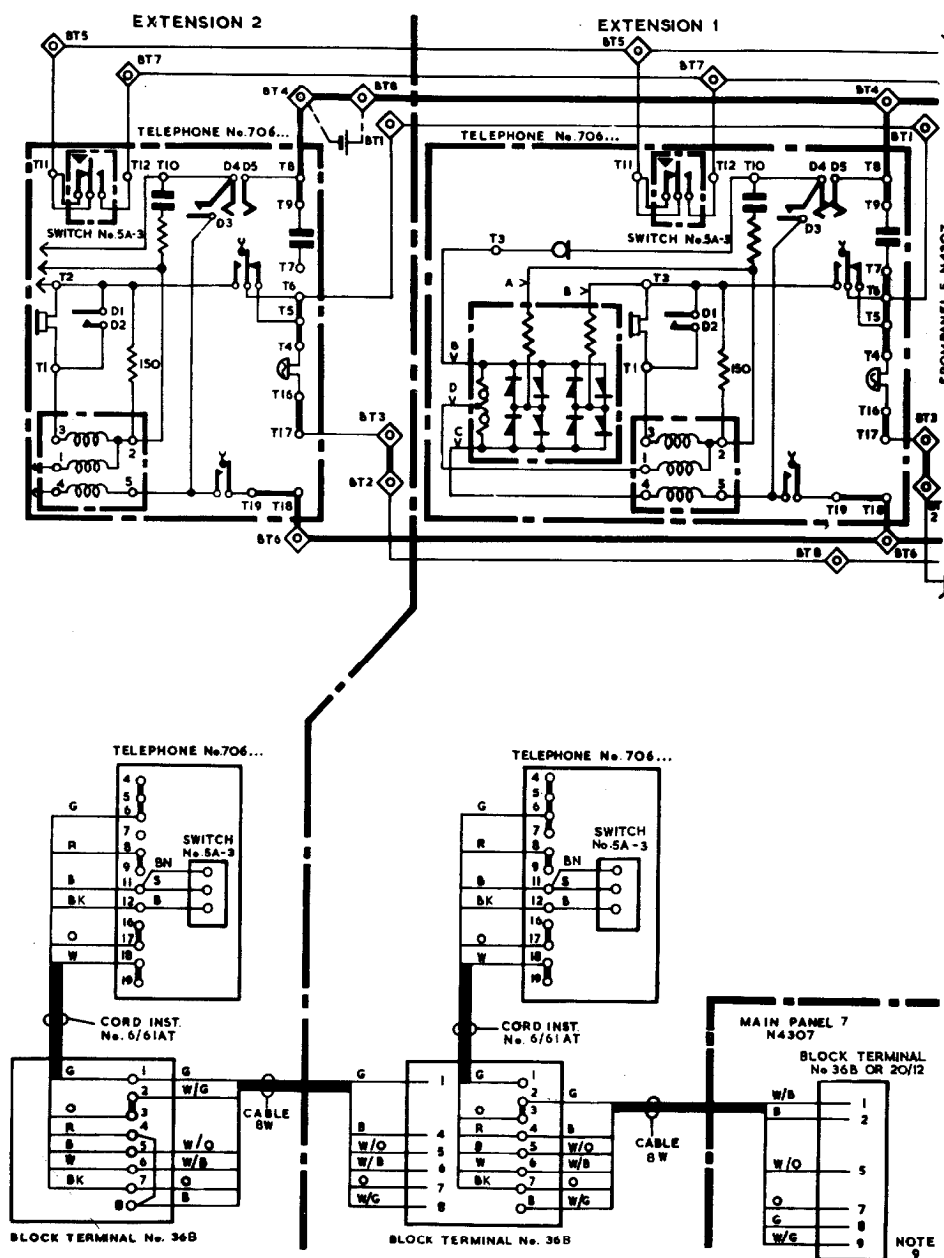
FIG. 2. EXTENSIONS FROM BELL SET No. 20.
