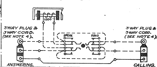
FIG. 3. PRIVATE WIRE OR TIE LINE WITHOUT EXCHANGE FACILITIES.
