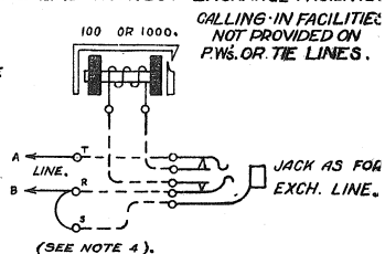
FIG. 3. PRIVATE WIRE OR TIE LINE WITHOUT EXCHANGE FACILITIES.
