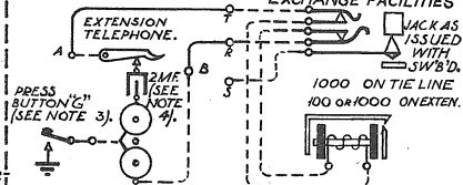
FIG 3 CORD CIRCUIT.
