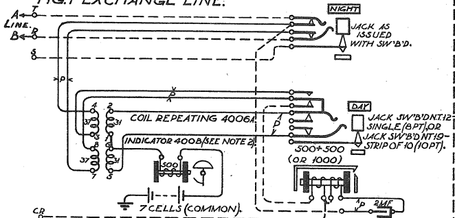
FIG. 1 EXCHANGE LINE.
