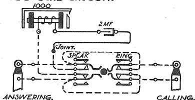
FIG 3 CORD CIRCUIT.
