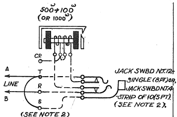
FIG. 1. EXCHANGE LINE.
