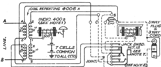
FIG.3. PRIVATE WIRE OR TIE LINE WITHOUT EXCH. FACILITIES (CALLING IN FACILITIES NOT PROVIDED)
