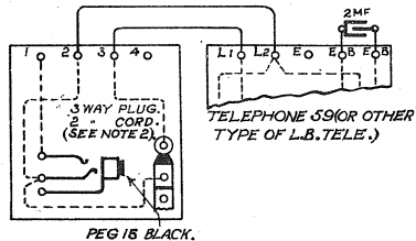
FIG.3. PRIVATE WIRE OR TIE LINE WITHOUT EXCH. FACILITIES (CALLING IN FACILITIES NOT PROVIDED)
