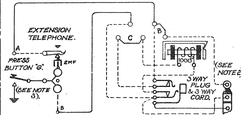
FIG.3. PRIVATE WIRE OR TIE LINE WITHOUT EXCH. FACILITIES (CALLING IN FACILITIES NOT PROVIDED)
