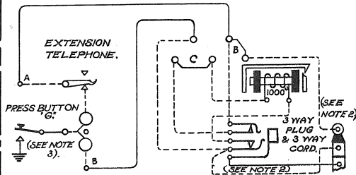
FIG. 3. PRIVATE WIRE OR TIE LINE
