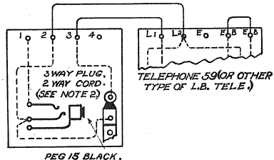
FIG. 4. OPERATORS TELEPHONE.
