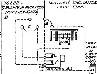
FIG. 3. PRIVATE WIRE OR TIE LINE
