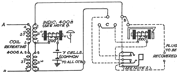
FIG. 3. PRIVATE WIRE OR TIE LINE
