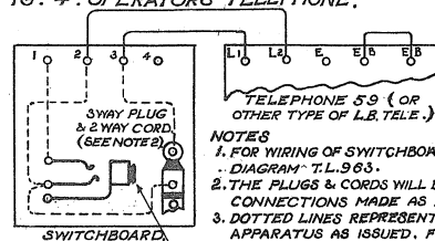
FIG. 4. OPERATORS TELEPHONE.
