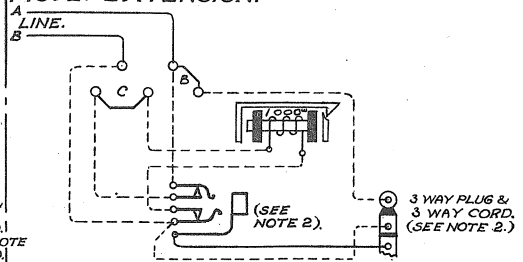
FIG. 4. OPERATORS TELEPHONE.
