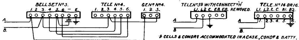
CONNECTIONS FOR DIFFERENT TELEPHONES AT EXT. N°.
