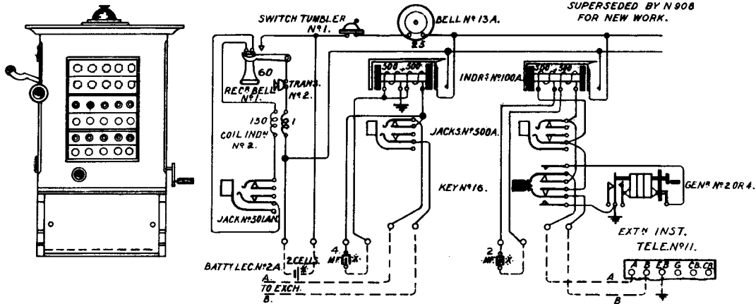
CONNECTIONS FOR DIFFERENT TELEPHONES AT EXT. N°.
