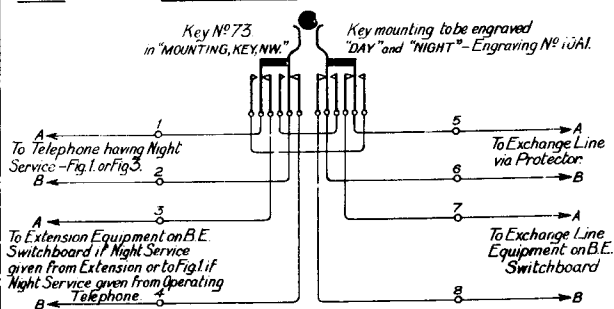
FIG. 4. NIGHT SERVICE KEY.
