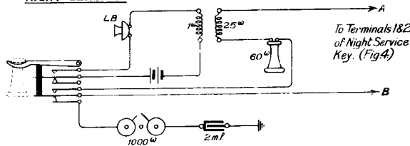
FIG. 3. TYPICAL TELEPHONE AT EXTENSION HAVING NIGHT SERVICE.
