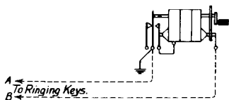
FIG. 2. SWITCHBOARD GENERATOR WHEN NIGHT SERVICE REQUIRED FROM EXTENSION.
