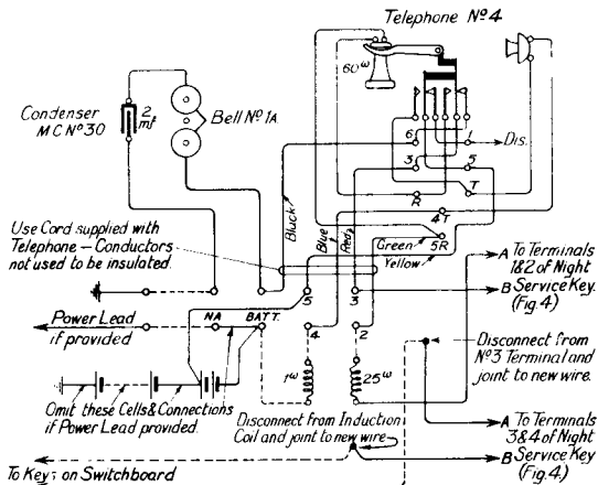
FIG. 2. SWITCHBOARD GENERATOR WHEN NIGHT SERVICE REQUIRED FROM EXTENSION.
