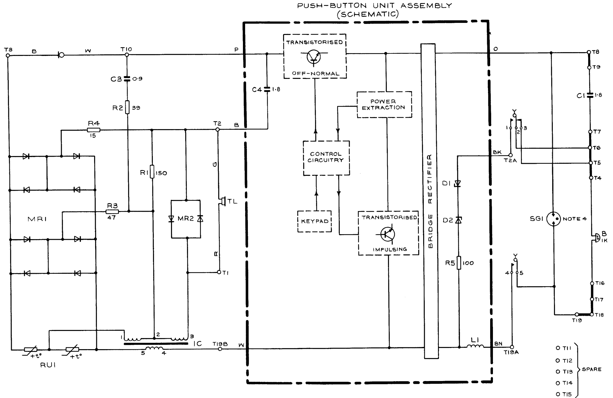
FIG.2 2,3 AND 4/758 CIRCUIT DIAGRAM SHOWING CONNEXIONS AS ISSUED
