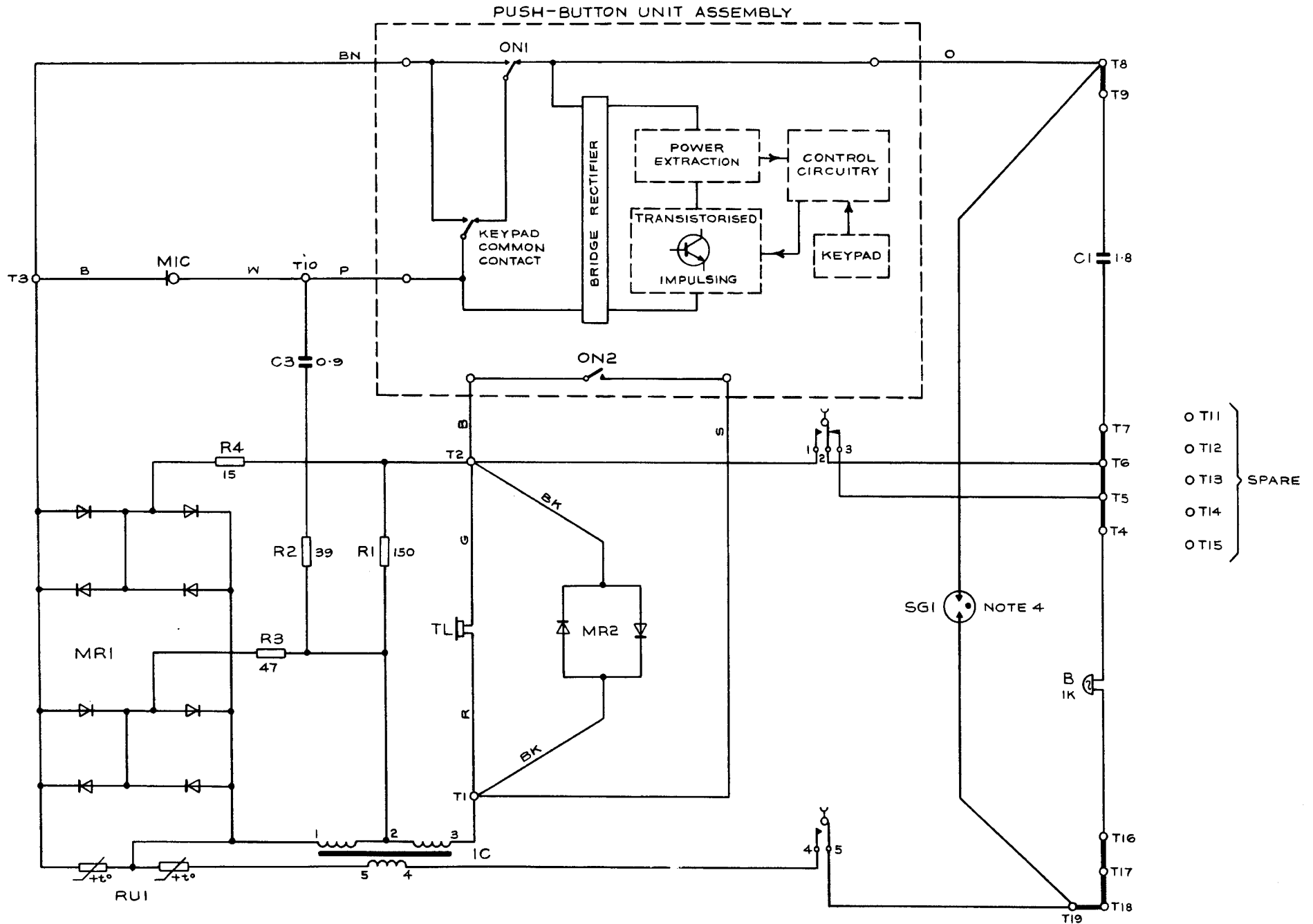
FIG.1 1/758 CIRCUIT DIAGRAM SHOWING CONNEXIONS AS ISSUED
