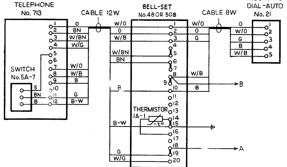
FIG. 3 SHARED SERVICE LINES
