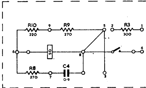
WIRING OF RELAY No.337A
