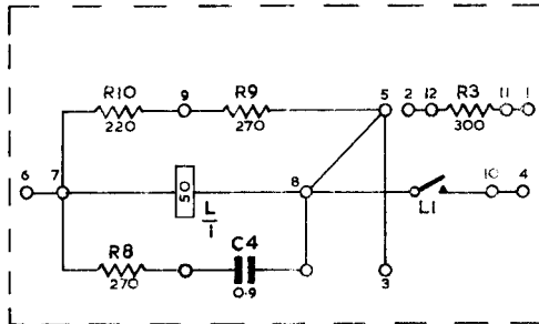
WIRING OF RELAY No. 337A
