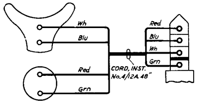
FIG.4. TRANSMITTER No. 23 & 23A, WITH PLUG No.406.
