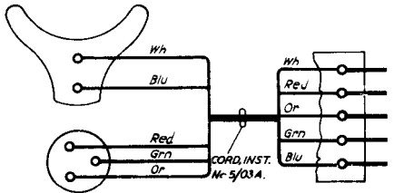
FIG.3. TRANSMITTER No. 23 & 23A, WITH PLUG No.501.
