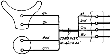
FIG.4. TRANSMITTER No. 23 & 23A, WITH PLUG No.406.
