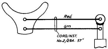
FIG.3. TRANSMITTER No. 23 & 23A, WITH PLUG No.501.
