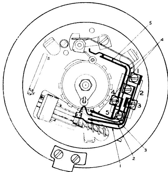
REAR VIEW SHOWING SPRING CONNEXIONS
