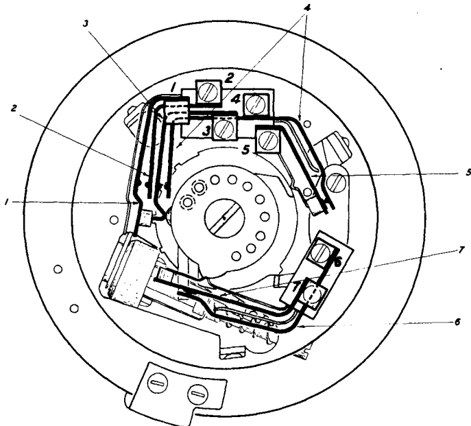
REAR VIEW SHOWING SPRING CONNEXIONS.
