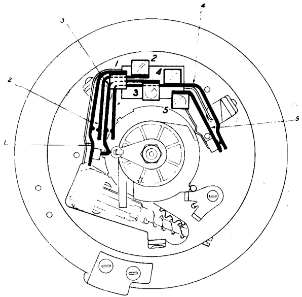
REAR VIEW SHOWING SPRING CONNEXIONS
