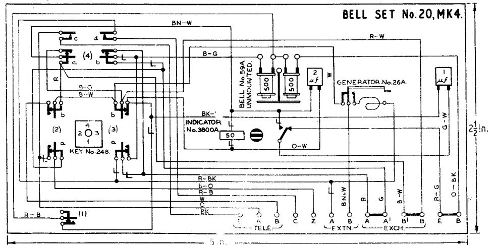
THE LABEL DIAGRAM TO BE REDUCED TO DIMENSIONS GIVEN.
