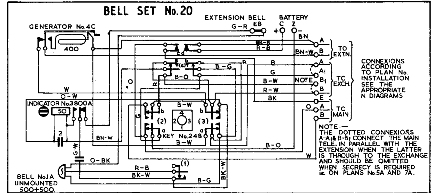
THE ABOVE WIRING DIAGRAM IS FOR MK1,2,3 AND EARLY SUPPLIES OF MK 4 BELL SET.
