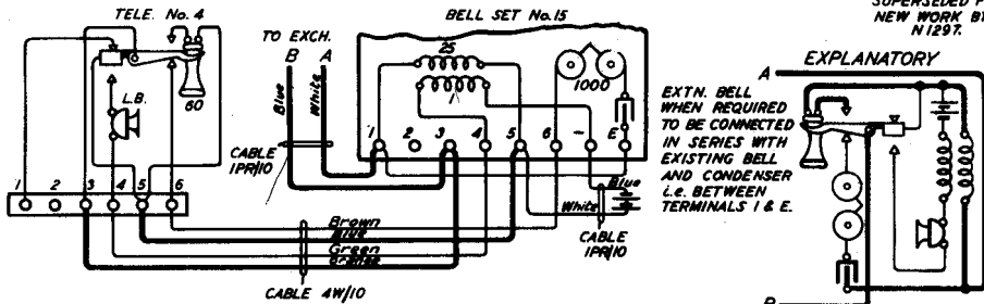
FIG.(2) CONNEXIONS FOR DIRECT EXCHANGE LINE MAGNETO SYSTEM (CONDENSER)
