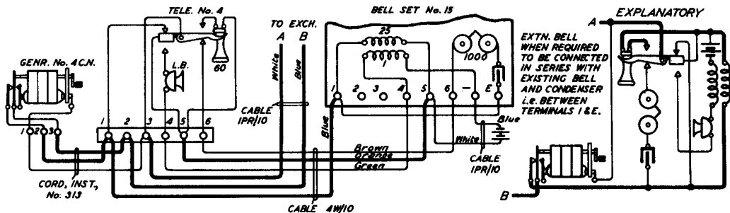
FIG.(2) CONNEXIONS FOR DIRECT EXCHANGE LINE MAGNETO SYSTEM (CONDENSER)
