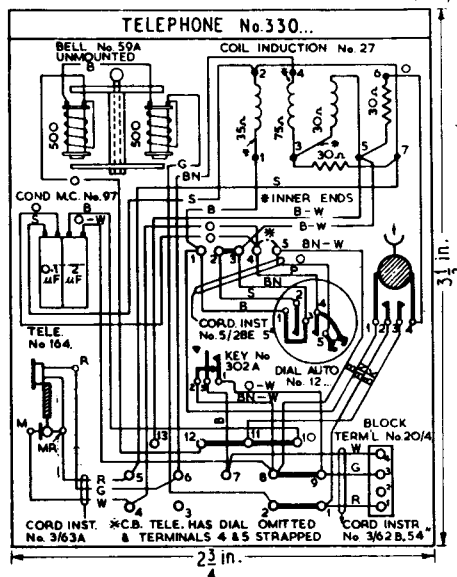
LABEL DIAGRAM TO BE TO DIMENSIONS GIVEN
