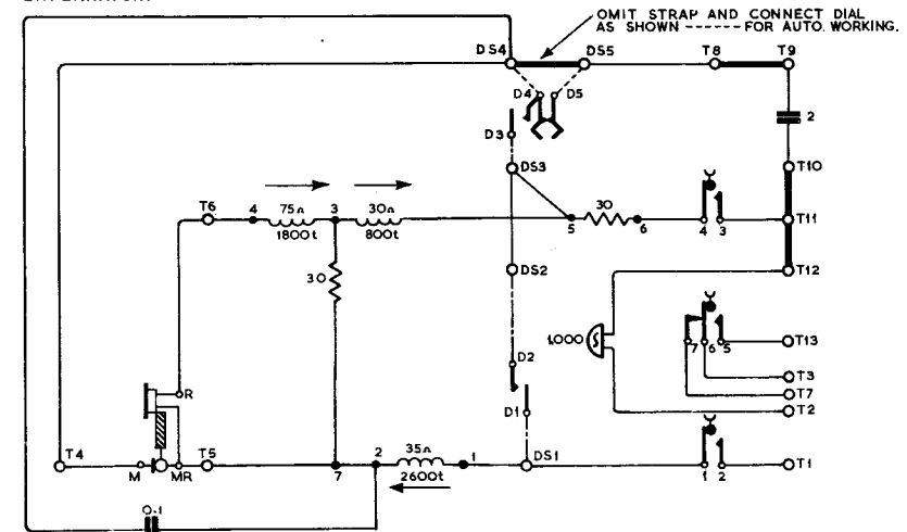
→ Indicates direction of windings on coil, induction.
