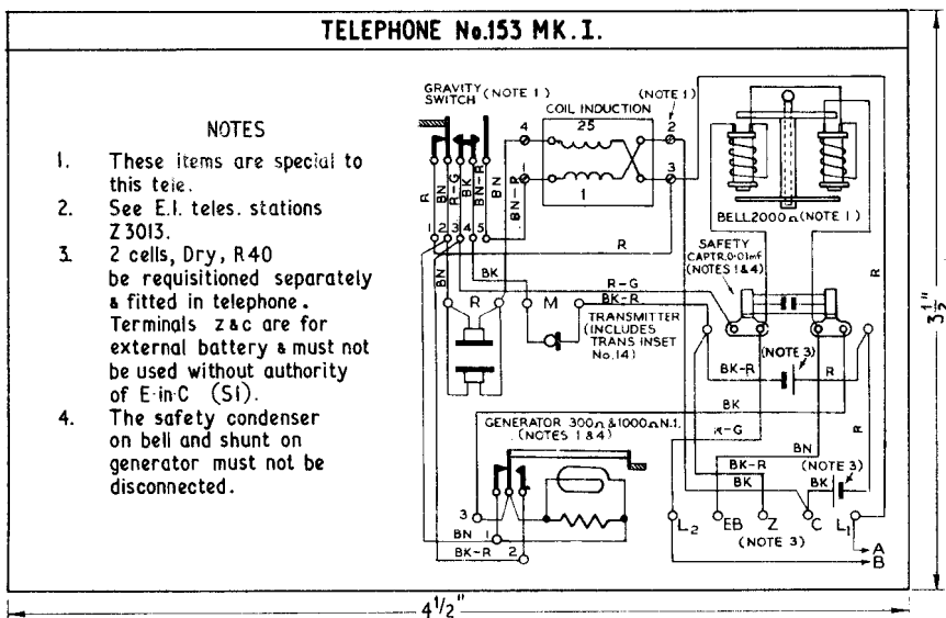
WIRING DIAGRAM
