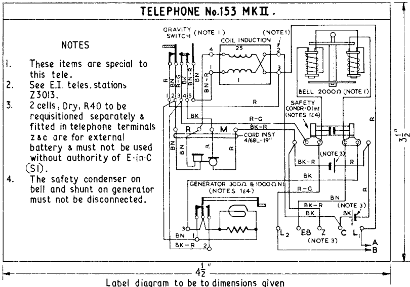
WIRING DIAGRAM
