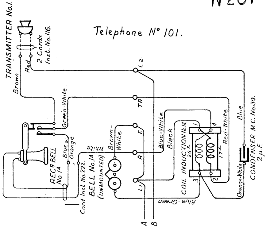
WIRING OF TELEPHONE No. 101
