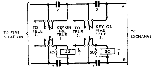
FIG. 3. SERIES ARRANGEMENT OF FIRE TELEPHONES.
