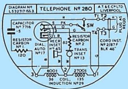
Wiring arrangements
