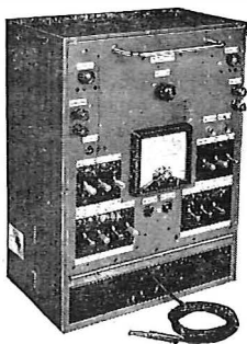
TESTER AT 5422 Manufactured for the G.P.O. and used for checking P.O. telephone lines.
