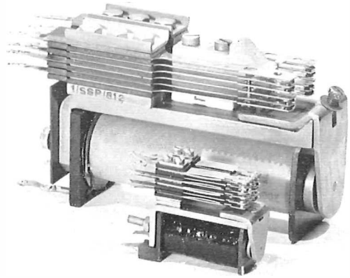
This picture shows the miniature relay (now named the Post Office type 16 relay) compared with the 3,000 type relay it replaced at Balham.
