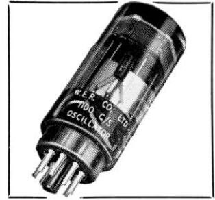
This fixed frequency oscillator is constructed on a standard octal base and encapsulated in epoxy resin.
