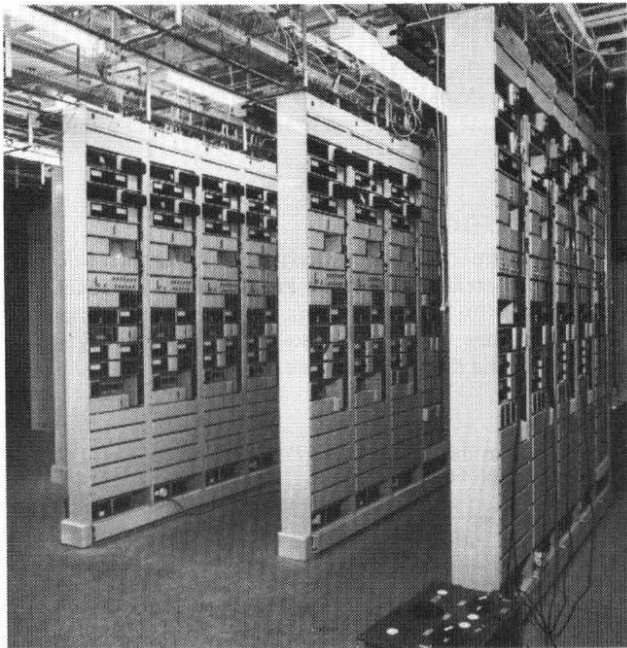
FIG. 5—The conclave equipment installation at High Wycombe (Equipment for the 60 MHz network was manufactured and installed by PYE/TMC in association with Philips Telecommunicate Industrie BV)
