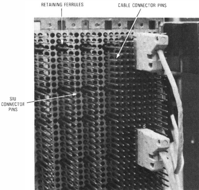
FIG. 11—Cable connector
