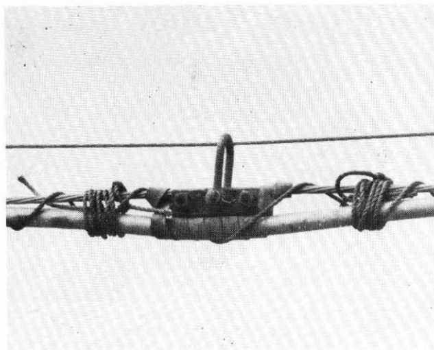
FIG. 3—Type of clamp adopted
