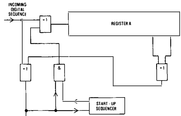
FIG. 6—Alternative design of improved error-detector
