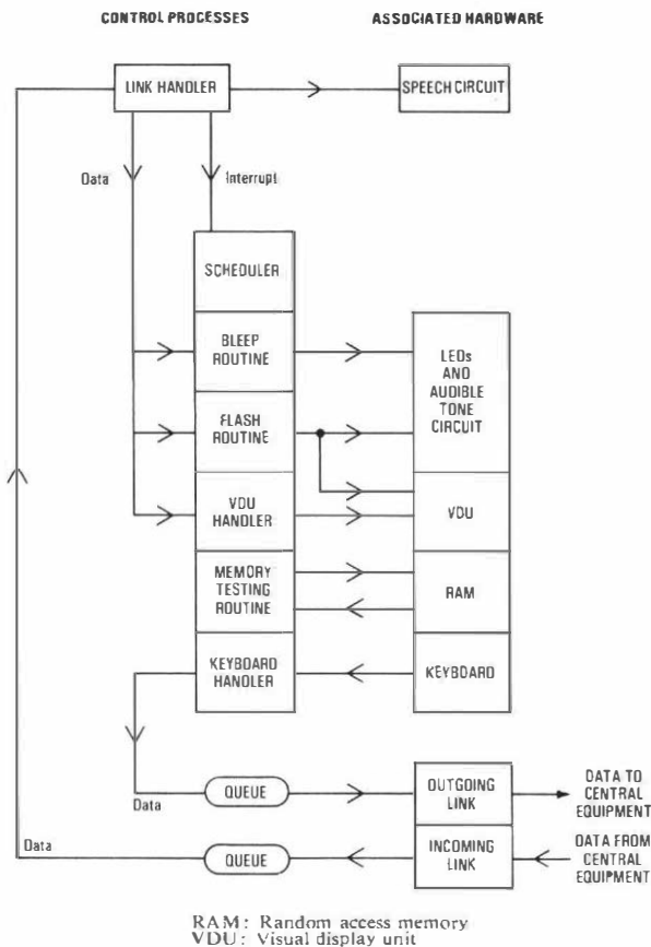
FIG. 6—Block diagram of the console control structure
