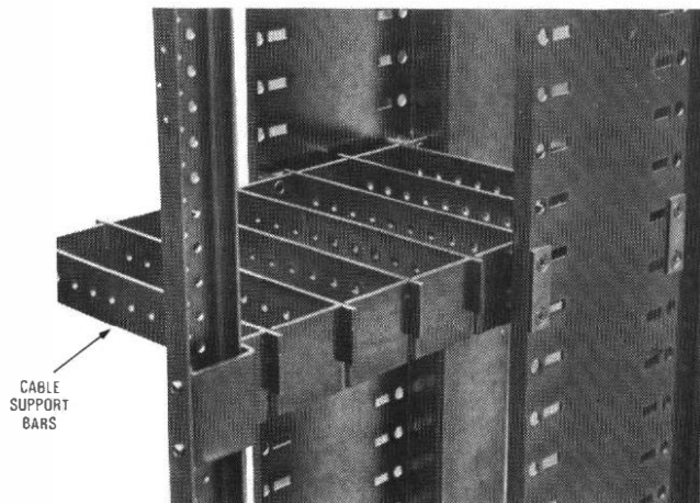
FIG. 13—Inter-rack spacing arrangement
