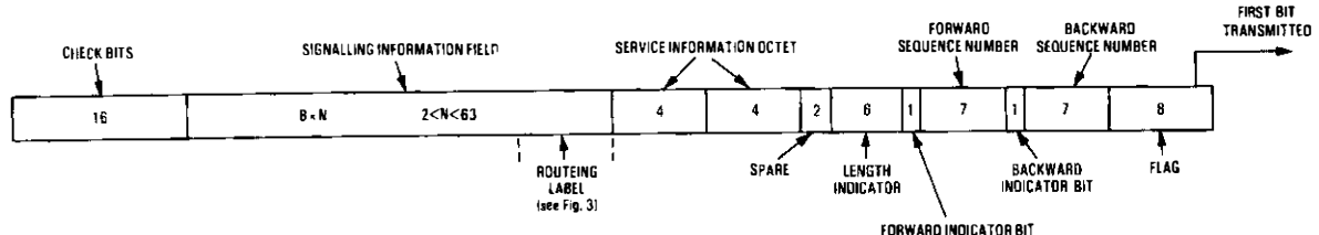
FIG. 1—Format of a message signal unit
