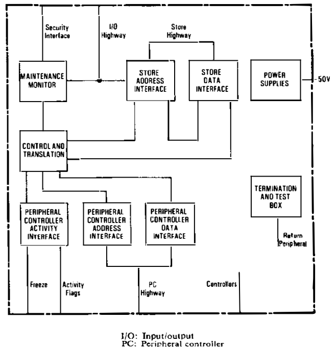
FIG. 4—Block diagram of the direct memory access system
