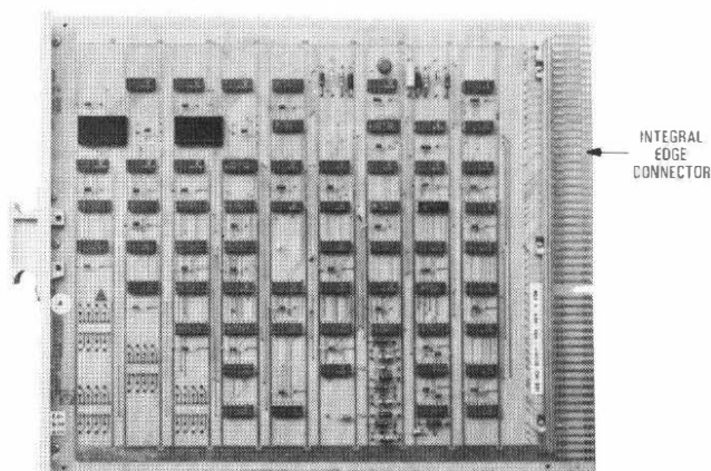
FIG. 9—A planar slide-in unit
