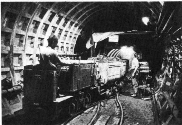
FIG. 7—Chamber at the foot of the work shaft with a train of skips leaving the air lock
