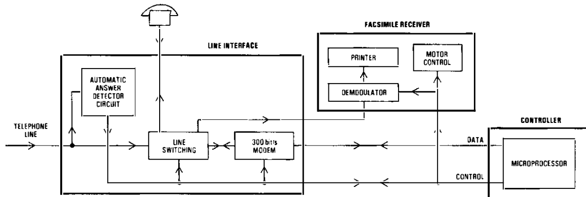
FIG. 5—Receiver terminal
