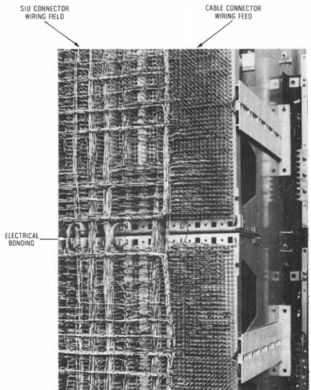
FIG. 6—Wiring of double shelf
