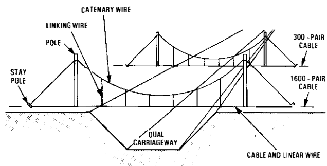
FIG. 2—Elevation of catenary support across dual carriageway
