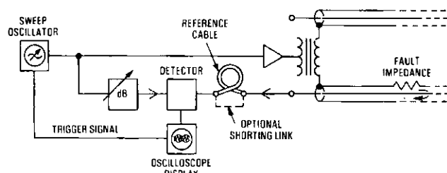
FIG. 7—Swept-frequency outer-injection crosstalk measurement technique
