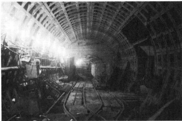
FIG. 6—The main enlargement (the west tunnel junction can be seen on the right-hand side of the photograph)
