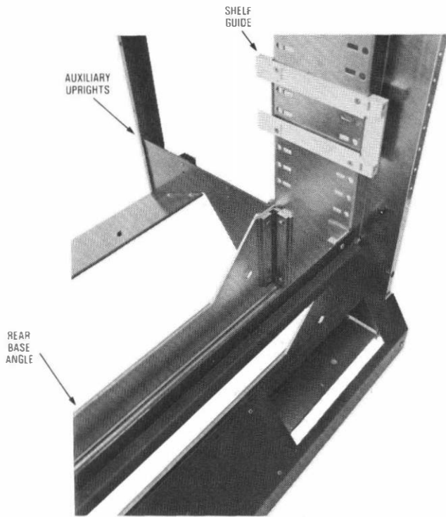
FIG. 3—Rack base
