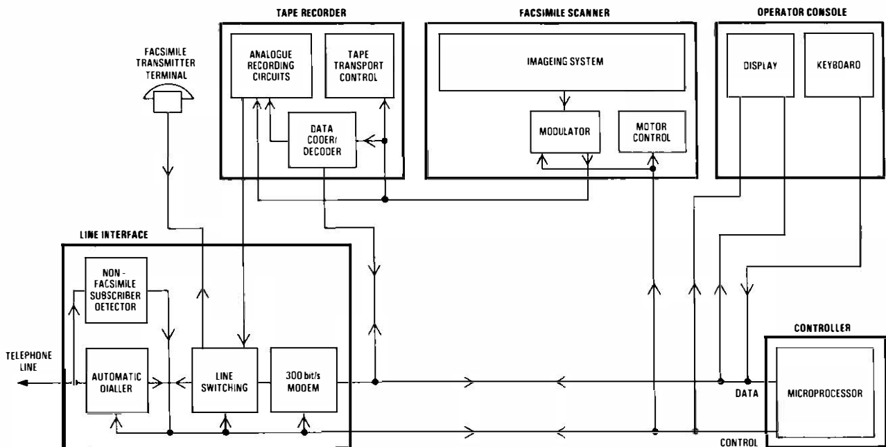
FIG. 4—Transmitter terminal
