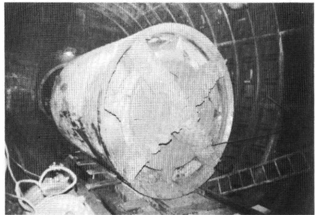
FIG. 4—Digger shield (at the end of its drive) showing the cutting face
