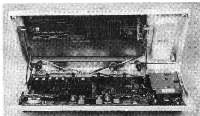
FIG. 2—Console in opened position
