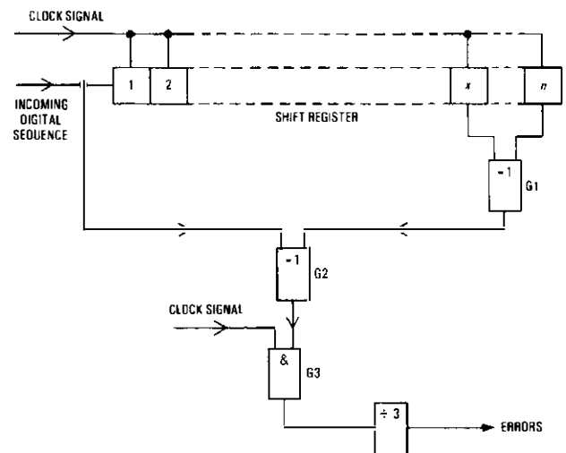
FIG. 3 Basic error-detector
