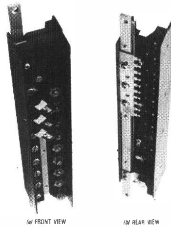
FIG. 12—Fuse mounting
