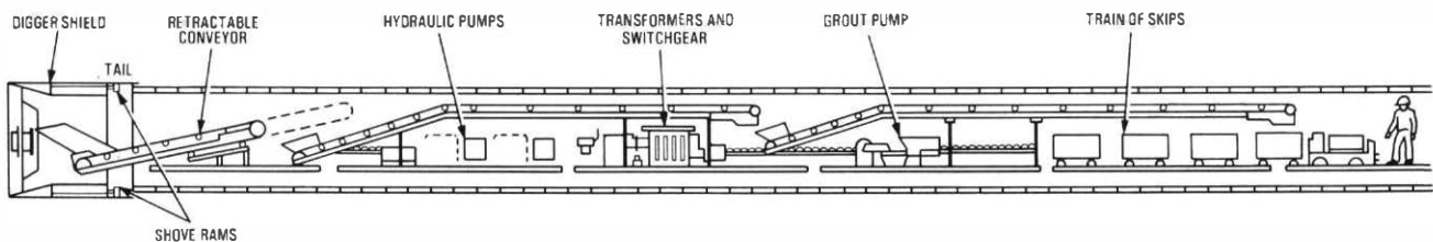
FIG. 3—Sectional drawing of the Sir Robert McAlpine full-face tunnelling machine
