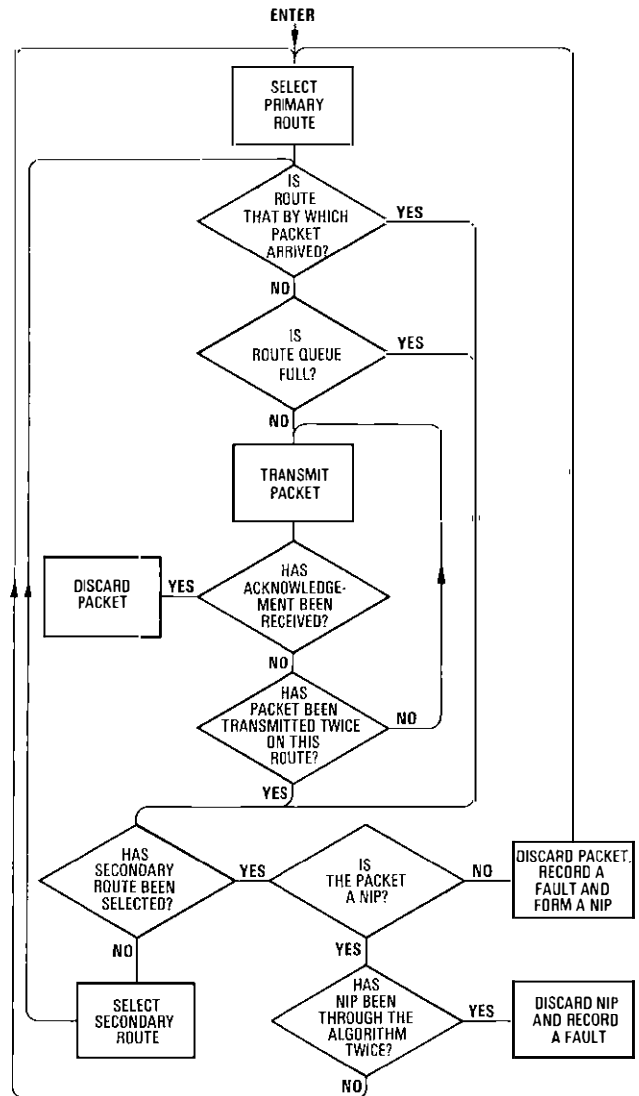
FIG. 16- Routing algorithm
