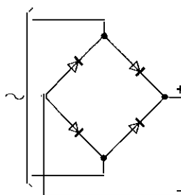
SINGLE-PHASE BRIDGE RECTIFIER
