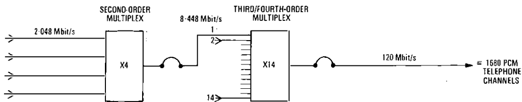
FIG. 2—Block diagram of multiplex equipment
