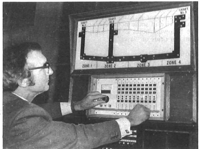
Alarm-indicating and gas-monitoring panels (By courtesy of Becorit (Great Britain) Ltd.)
