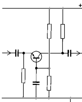
COMMON-BASE RC COUPLED AMPLIFYING STAGE
