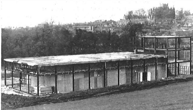
Wooden cocoon within the steel framework, 1 month before equipment installation commenced
