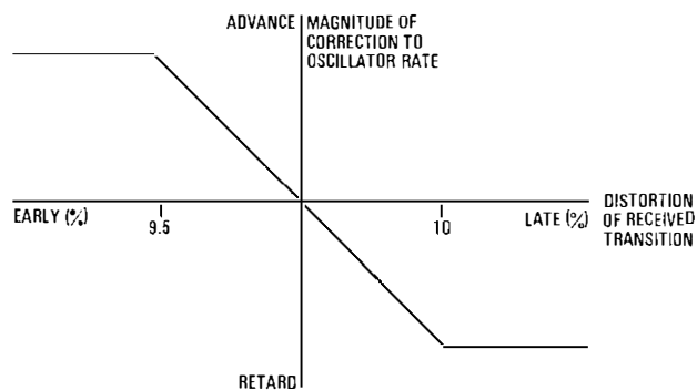
FIG. 9—Tester TG 2402 synchronizer characteristics
