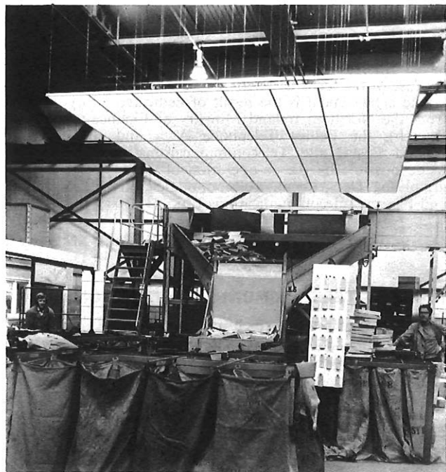
Diffuser suspended over the concentrator's working area
