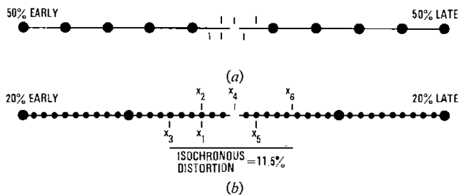
(a) Displayed range 50% early to 50% late (b) Displayed range 20% early to 20% late
