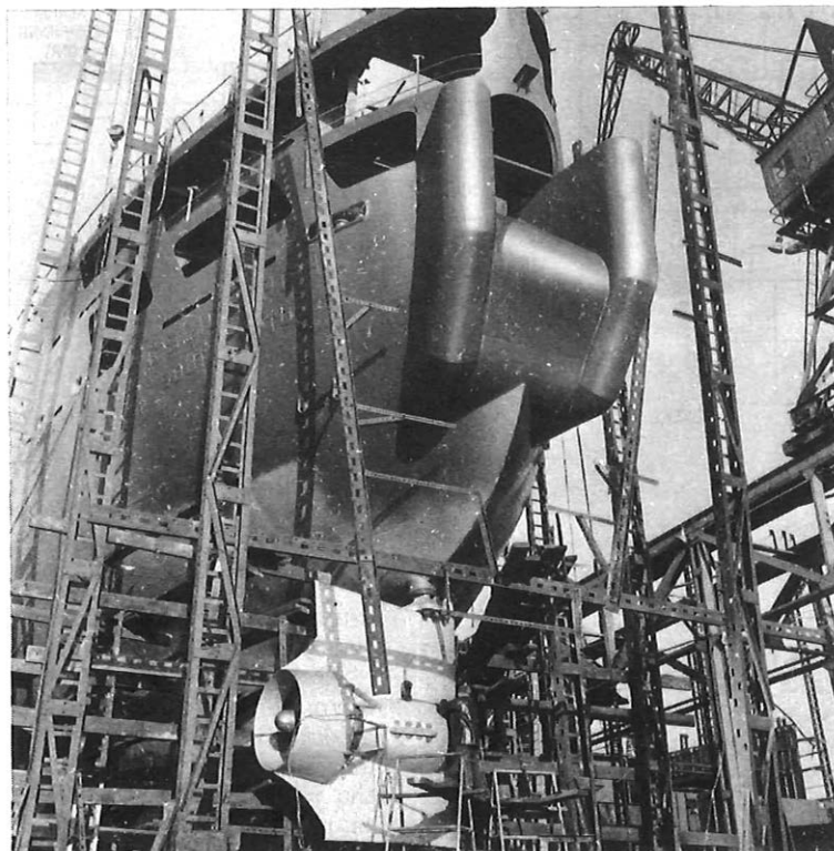
Fig. 1—Stern of CS Monarch with power rudder fitted, shortly before the launch date
