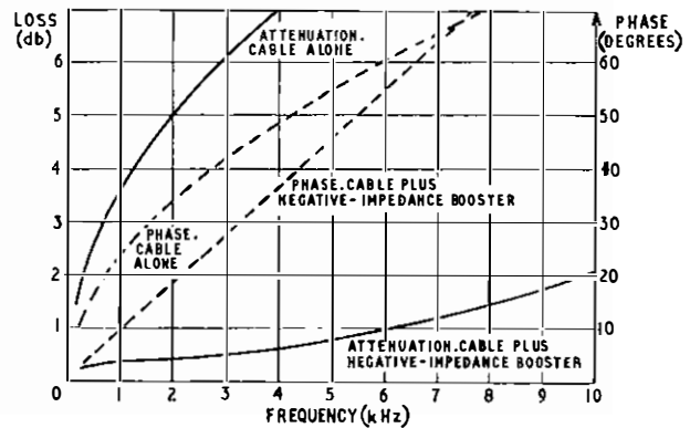
FIG. 11—Attenuation and phase coefficients for a 2,000 yd section of 0.4 mm cable
