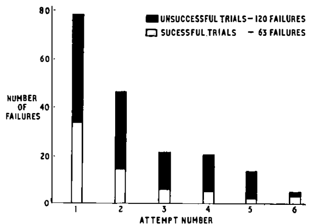
FIG. 5—Second and subsequent occurrences of intermittent faults—number of failures recorded at each of the six test attempts
