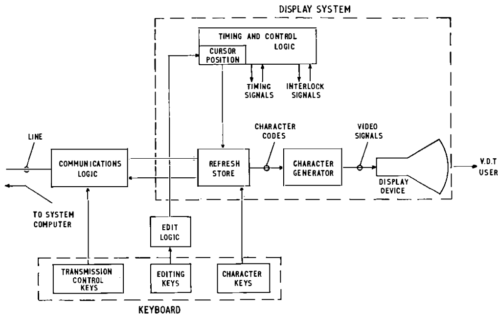
FIG. 3—Block diagram of the alpha-numeric v.d.t.
