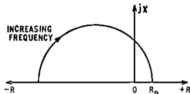
FIG. 8—Impedance plot for the negative-impedance booster
