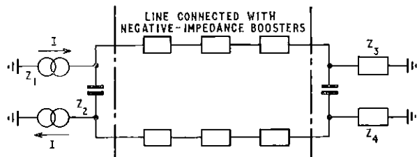
FIG. 9—Power-feed arrangement for the negative-impedance booster line
