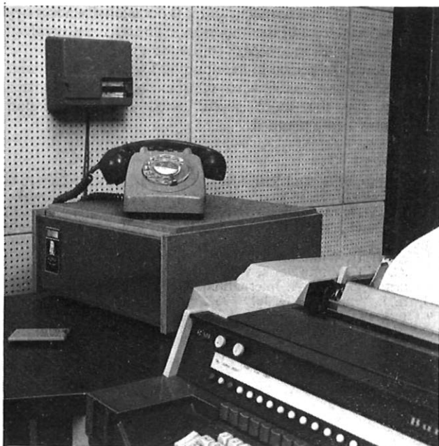
FIG. 3—Outstation showing Case No. 200, modem, standby telephone and the customer's terminal
