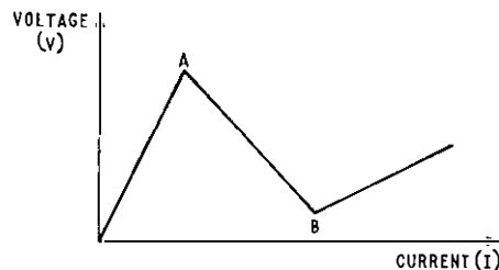
FIG. 5—Voltage/Current characteristic of a series-connected negative-impedance booster
