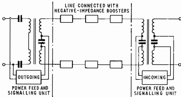
FIG. 10—Signalling arrangement for the negative-impedance booster line
