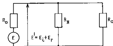
FIG. 3—Shunt-connected n.i.b.
