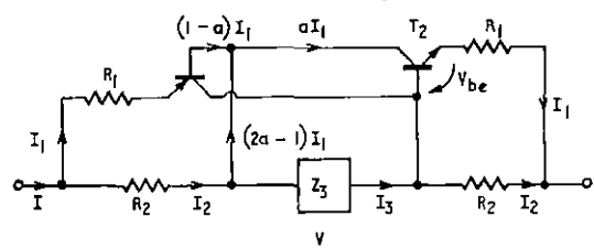
FIG. 14—Symmetrical negative-impedance booster circuit
