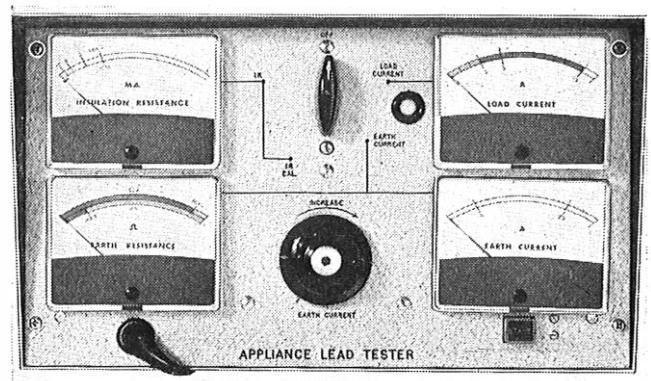
FIG. 2.—Front panel of prototype tester
