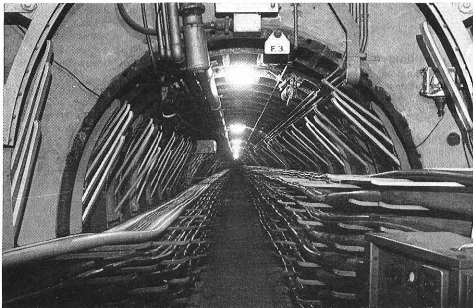
FIG. 2—Typical 7 ft diameter cable tube approximately half-filled
