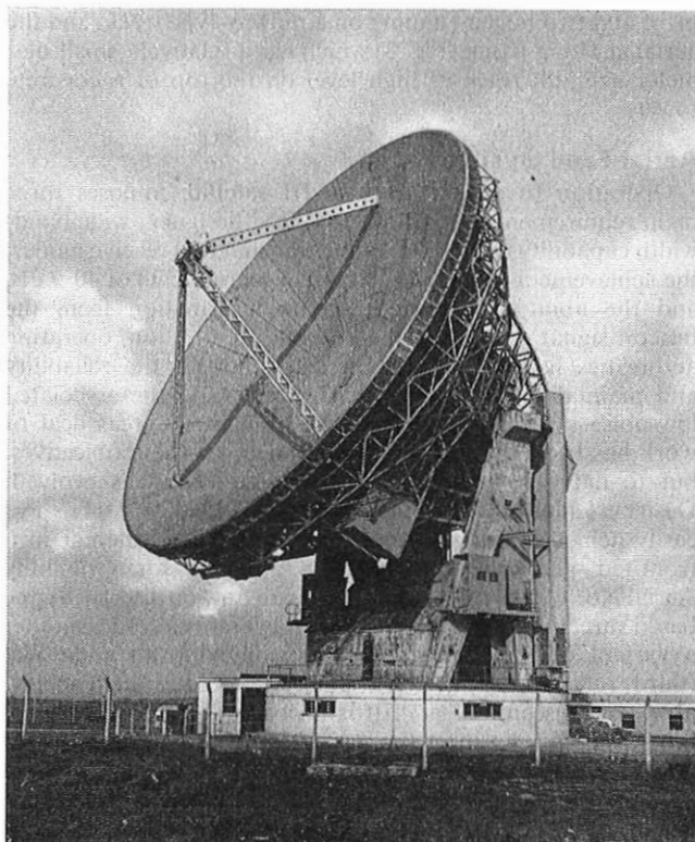
FIG. 1—Goonhilly Aerial No. 1. Built in 1961, modified in 1965 to give improved profile accuracy
