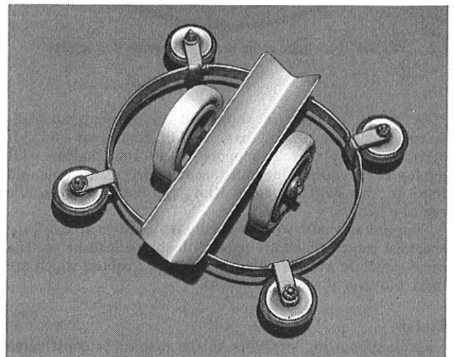
FIG. 9—Cabling trolley
