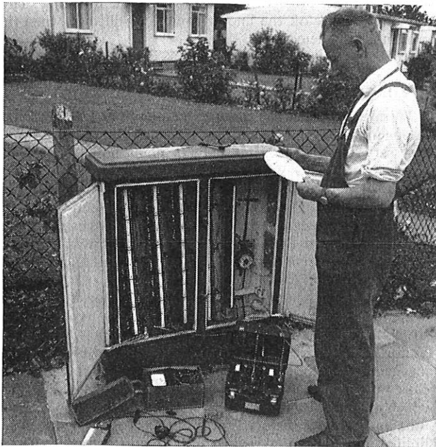
FIG. 4—Using Ohmmeter No. 18A and fault-locating slide-rule
