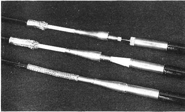
FIG. 2—Typical joints at the moulding stage
