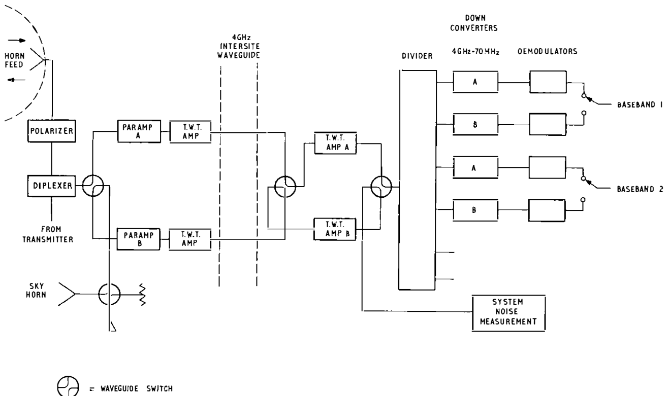
FIG. 5—Simplified block schematic diagram of receive equipment
