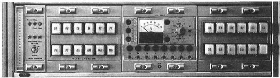
FIG. 8—Control panel
