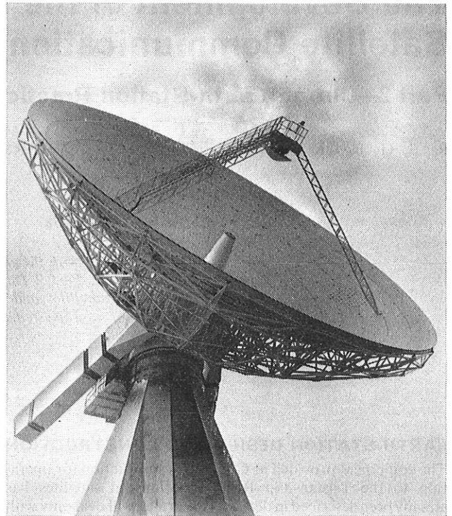
FIG. 3—Aerial at Hong Kong, built in 1969. The high-level azimuth track at the top of the concrete tower can be seen clearly.
