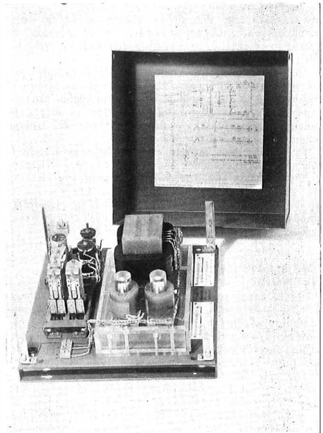
FIG. 2—Line Isolating Unit 1A
