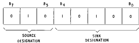
FIG. 6—Eight-bit instruction
