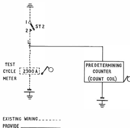
FIG. 2—Connexion of counter to traffic recorder.
