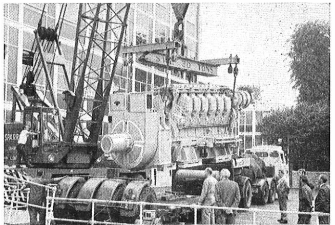
Diesel-engine generating set being lifted from transporter.
