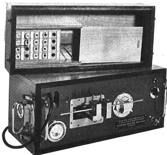
FIG. 1—RESISTANCE-BRAZING MACHINE
