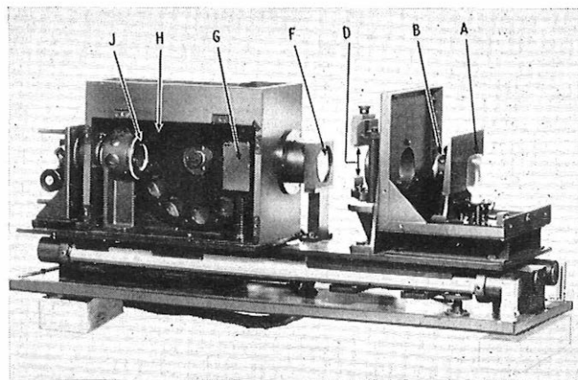
FIG. 3—TYPE 1 OPTICAL UNIT WITH INTERNAL COVERS REMOVED
