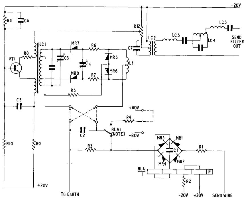
Note: Contact RLA1 is shown operated FIG. 4—OSCILLATOR-MODULATOR
