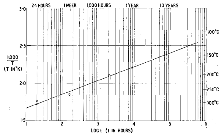
FIG. 5--LIFE PREDICTION LINE
