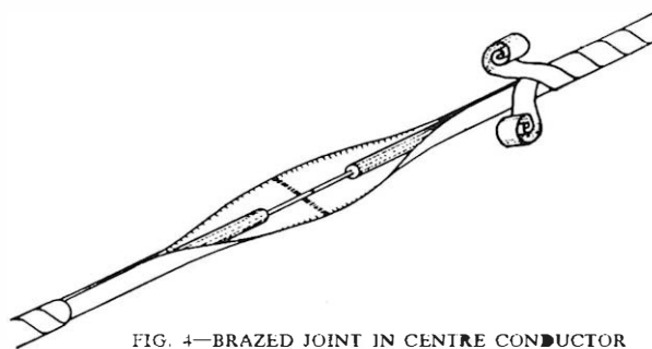
FIG. 4—BRAZED JOINT IN CENTRE CONDUCTOR
