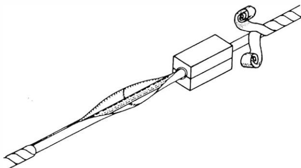
FIG. 5—RESTORATION OF OUTER CONDUCTOR
