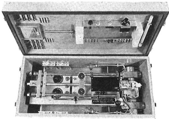
FIG. 3—MOULDING MACHINE IN CARRYING CASE
