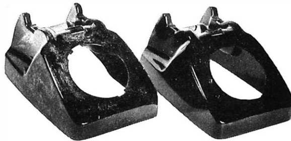
The right-hand case was wiped with Cetrimide solution, the left-hand case was untreated. Both were then polished and exposed to dust (cotton lint). THE EFFECT OF ANTI-STATIC TREATMENT OF TELEPHONE MOULDINGS
