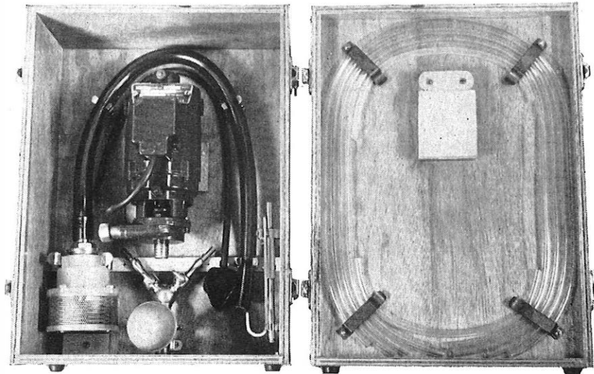
FIG. 6--COOLING-WATER UNIT IN CARRYING CASE
