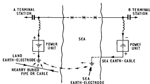
FIG. 1—TYPICAL SUBMARINE-CABLE D.C. POWER-FEEDING ARRANGEMENTS
