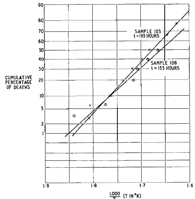
FIG. 3—165-HOUR STEP-STRESS TESTS WITH 30 TRANSISTORS IN EACH SAMPLE
