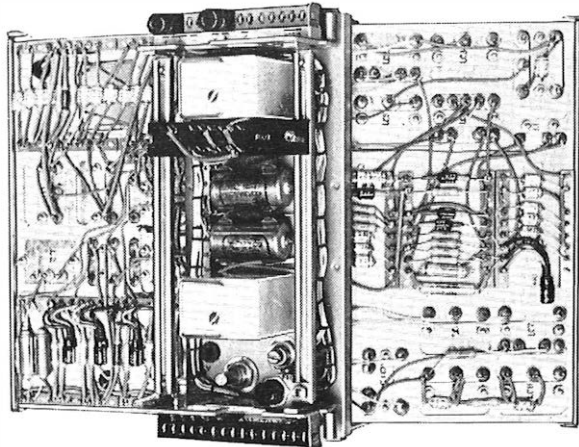
FIG. 3—CHANNEL PANEL WITH SIDE LEAVES OPEN
