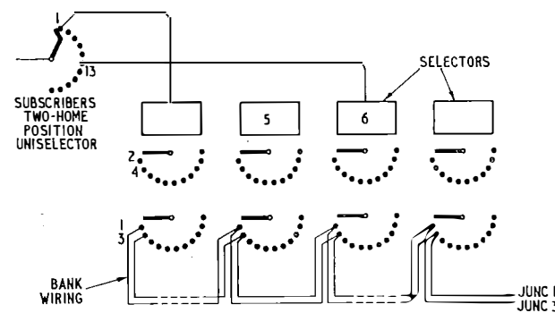
(b) Transposition in Bank Wiring.
