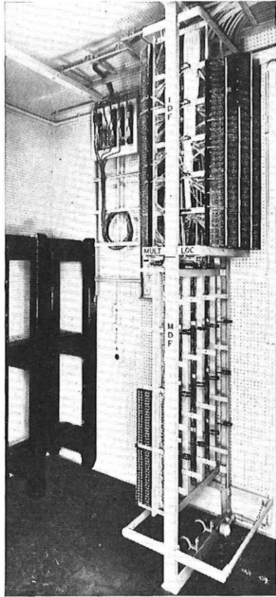
FIG. 5—COMBINED MAIN AND INTERMEDIATE DISTRIBUTION FRAME
