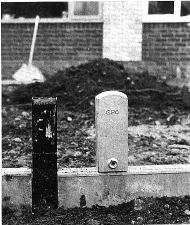
ABOVE-GROUND JOINTING POST
