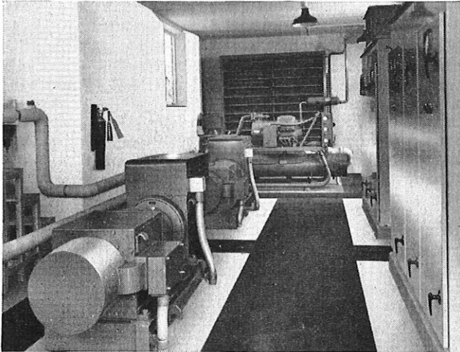
Two buffer alternators in the foreground with associated control cabinets to the right. In the background can be seen the high-speed compressor and air-cooled condenser. These are rated at 13 tons of refrigeration.
