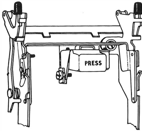
FIG. 4—SINGLE-PUSH-BUTTON UNIT
