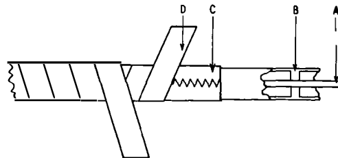
(a) Worm-Type Coaxial Pair
