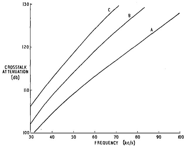
FIG. 9--COMPARISON OF EFFECTS OF DIFFERENT METHODS OF APPLYING OUTER STEEL TAPES
