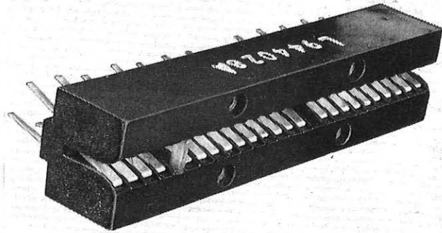
FIG. 7—SOCKET WITH NYLON POLARIZING DEVICE
