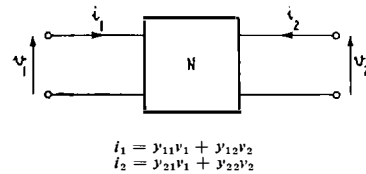
FIG. 10—ILLUSTRATING THE y -PARAMETERS OF A NETWORK
