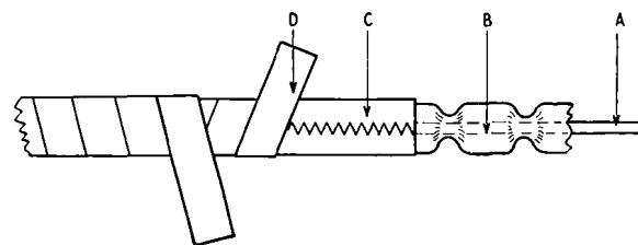
(c) Disk-Type Coaxial Pair
