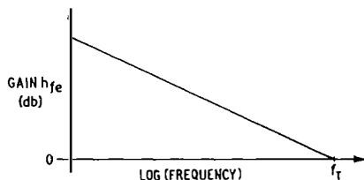
FIG. 3—FREQUENCY RESPONSE OF IDEAL TRANSISTOR
