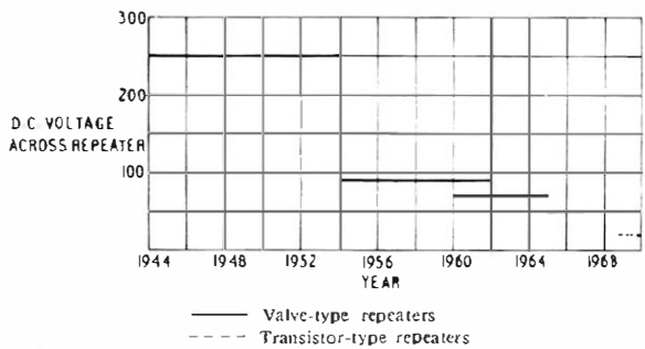
FIG. 6—D.C. VOLTAGE REQUIREMENTS OF BRITISH REPEATERS
