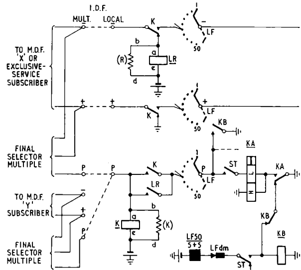
FIG. 8—SUBSCRIBER'S LINE CIRCUIT IN 50-POINT LINEFINDER SYSTEM
