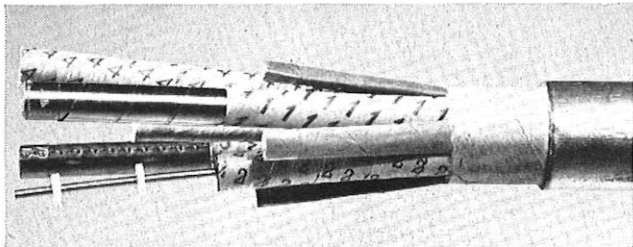
(a) Typical 375-type Coaxial Cable
