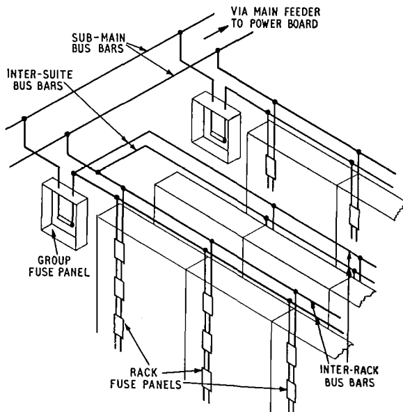
FIG. 1—TYPICAL BUS-BAR ARRANGEMENT
