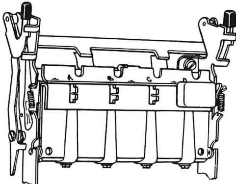
FIG. 5—MULTI-PUSH-BUTTON UNIT
