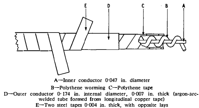
(a) Worm-Type Coaxial Pair
