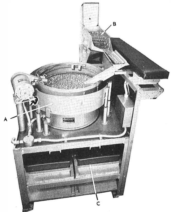
A—Second sorting unit B—Filling hopper and linear feeder C—Tray for sorted screws FIG. 1—SCREW-SORTING MACHINE
