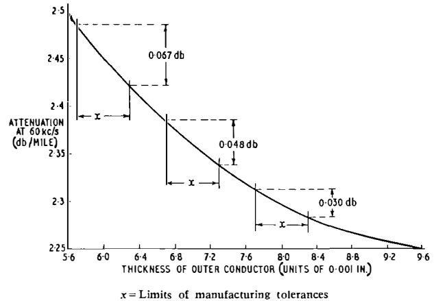
FIG. 4—RELATION OF ATTENUATION TO THICKNESS OF OUTER CONDUCTOR
