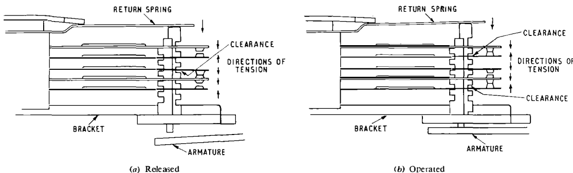
FIG. 7—SPRING-SET OPERATION
