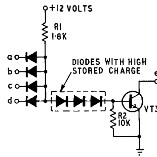
FIG. 32—TRANSISTOR-DIODE LOGIC
