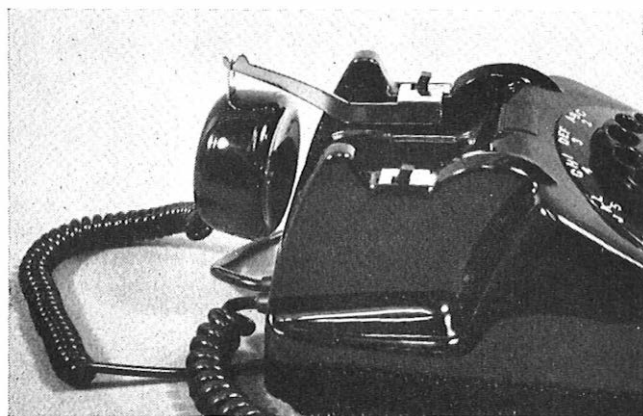
FIG. 1—WATCH RECEIVER AND BRACKET ON 700-TYPE TELEPHONE
