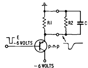
FIG. 40—P-N-P EMITTER FOLLOWER
