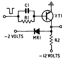
(a) Diode Clamp
