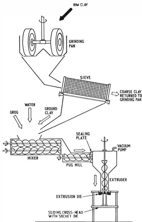
FIG. 3—DIAGRAM OF MIXING AND EXTRUDING MACHINES
