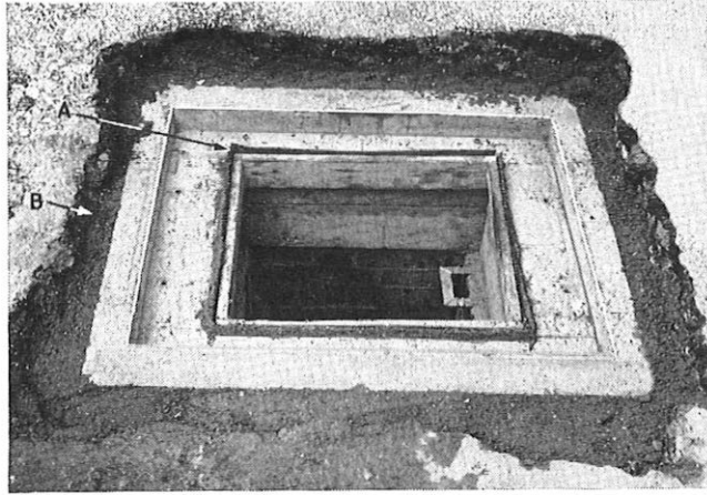
A—Rubber shuttering B—Dry concrete backfill
