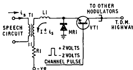
FIG. 36—CURRENT-CONTROLLED MODULATOR
