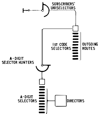
(a) Electromechanical A-Digit Selectors and Directors
