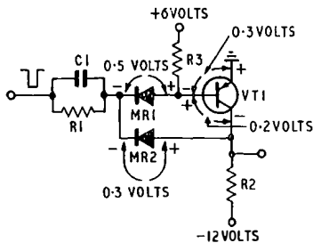
(b) Low-Dissipation Clamp
