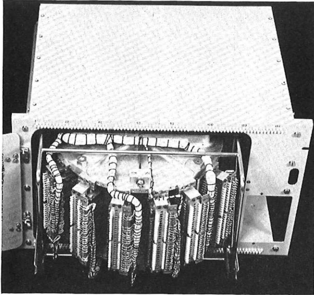
FIG. 1—MAGNETIC-DRUM STORE
