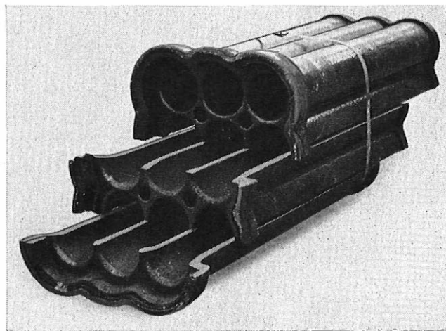
SPECIALLY-GROOVED 9-WAY MULTIPLE DUCT
