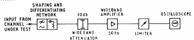
FIG. 4—BLOCK SCHEMATIC DIAGRAM OF CIRCUIT FOR NON-LINEARITY MEASUREMENTS AT RECEIVE END OF CHANNEL
