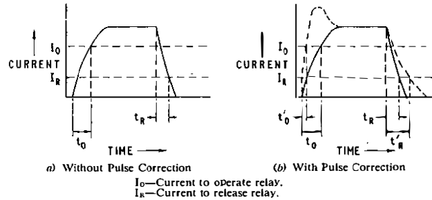
FIG. 10—PULSE CORRECTION IN V.F. RECEIVER
