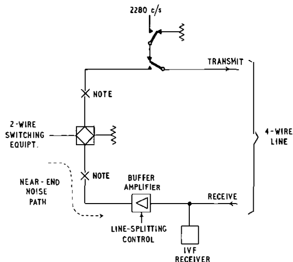
FIG. 1—SIGNALLING EQUIPMENT CONNECTED IN THE 4-WIRE LINE
