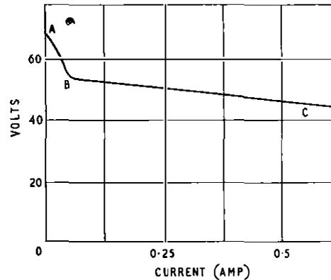
FIG. 2—OUTPUT-VOLTAGE/LOAD-CURRENT CHARACTERISTIC
