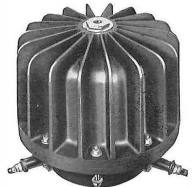
5 kW Type L.382 in cast aluminium. Frequency range 1.5-30 Mc/s, with VSWR better than 1.5
