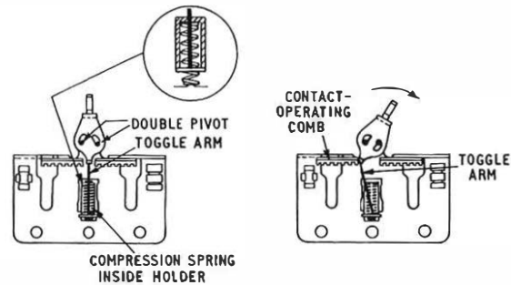
FIG. 2.—TOGGLE ACTION—DOUBLE-THROW KEY
