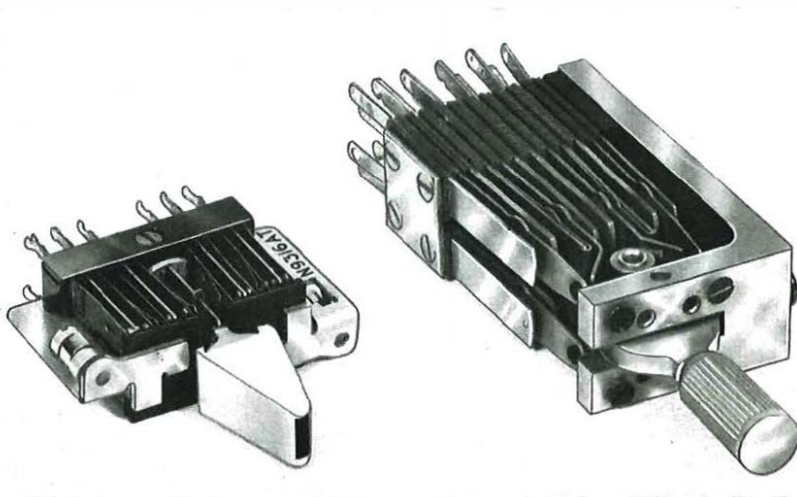
FIG. 1.—1,000-TYPE KEY AND STANDARD KEY
