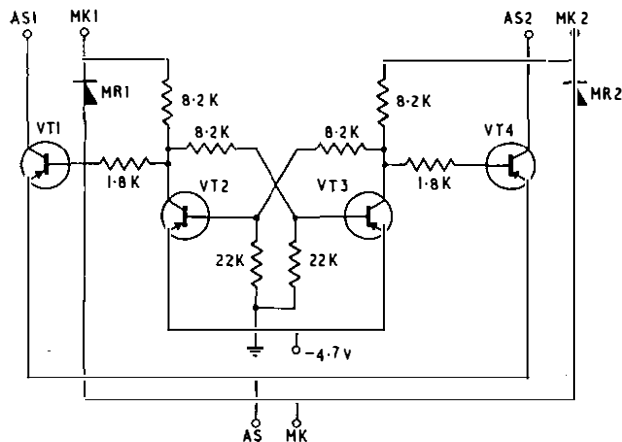
FIG. 7—BI-STABLE TRIGGER CIRCUIT
