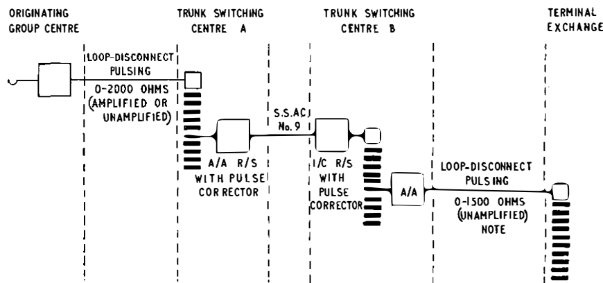
Note: 0-2,000 ohms (unamplified) where the terminal exchange equipment is 2,000-type. FIG. 2—TYPICAL OPERATOR ROUTING OVER S.S.A.C. No. 9 CIRCUIT
