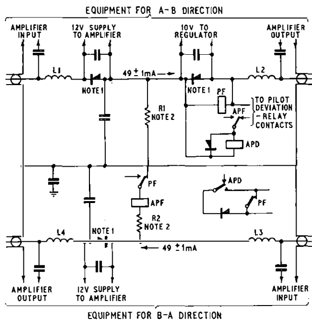
Notes: 1 Zener diode. 2 The sum of the values of R1 and R2 equal the resistance of the inner conductor to the end of the power-feeding section. FIG. 6—DEPENDENT REPEATER: POWER, ALARM AND SUPERVISORY CIRCUITS
