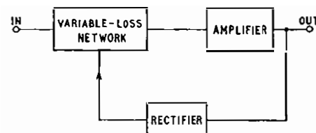
FIG. 1—BASIC CIRCUIT OF COMPRESSOR
