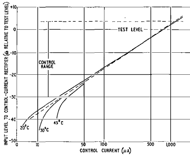
FIG. 7—CONTROL-CURRENT RECTIFIER: INPUT-LEVEL/CONTROL-CURRENT CHARACTERISTIC
