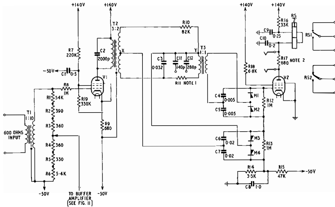
Notes: 1. Value of resistor R11 is chosen by manufacturer. 2. Resistor R17 is required for routine test purposes. FIG. 7—S.S.A.C. No. 9 V.F. RECEIVER
