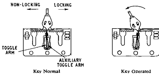
FIG. 4—LOCKING/NON-LOCKING ACTION
