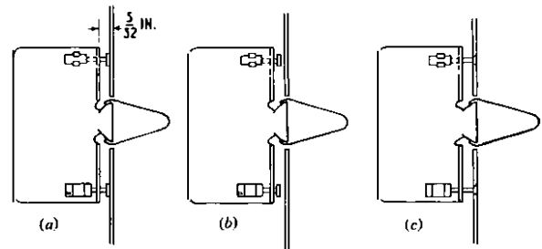
(a) 8 BA Studs Welded to Rear of Panel (b) 8 BA Studs Carried on Subsidiary Frame (c) 8 BA Screws Through Key Panel
