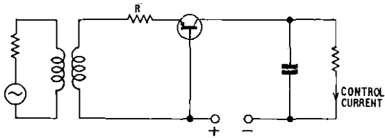
FIG. 6—CONTROL-CURRENT RECTIFIER
