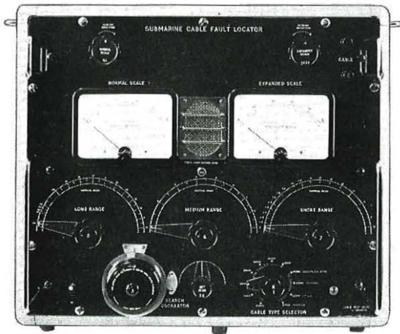
FIG. 1.—SUBMARINE-CABLE FAULT LOCATOR
