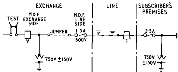
FIG. 10—PRE-1957 PROTECTIVE ARRANGEMENTS
