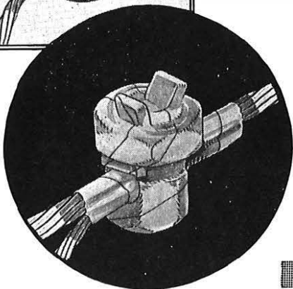
Copper-aluminium line tap coated with Denso Paste, wrapped in Denso Tape.
