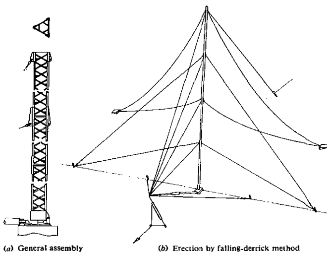
FIG. 5—CONSTRUCTION AND ERECTION OF MAST
