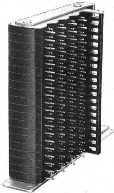
(b) Right-Hand Side FIG. 4—FUZE UNIT
