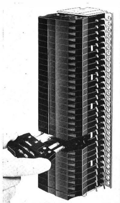
FIG. 1.—FUSE UNIT USED AT SPRINGPARK EXCHANGE
