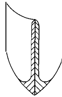
FIG. 3—PATTERN OF INDUCTION-HARDENED ZONE DUE TO EXCESSIVE TIME OF HEATING
