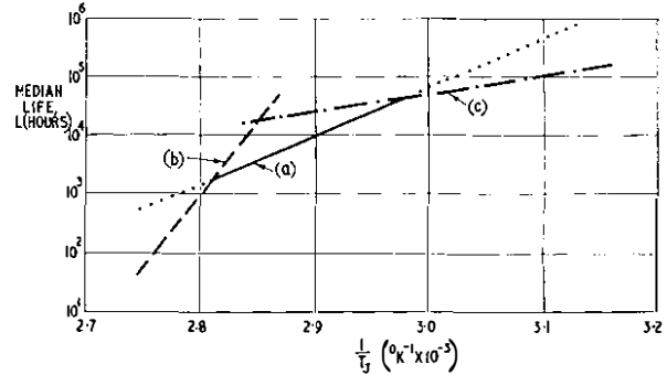
FIG. 4—SUPERPOSITION OF THREE LIFE LAWS OF THE FORM L = A \exp(B/T_J)
