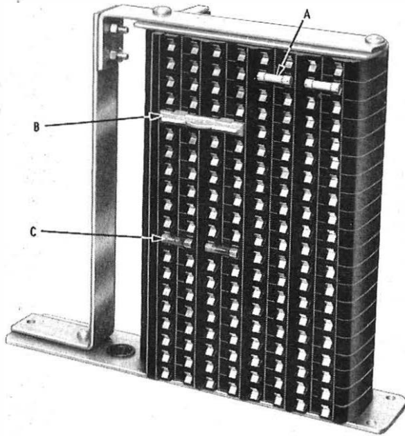
(a) Left-Hand Side showing Dummy Fuses (A), Fuse Covers (B), and Fuses (C)
