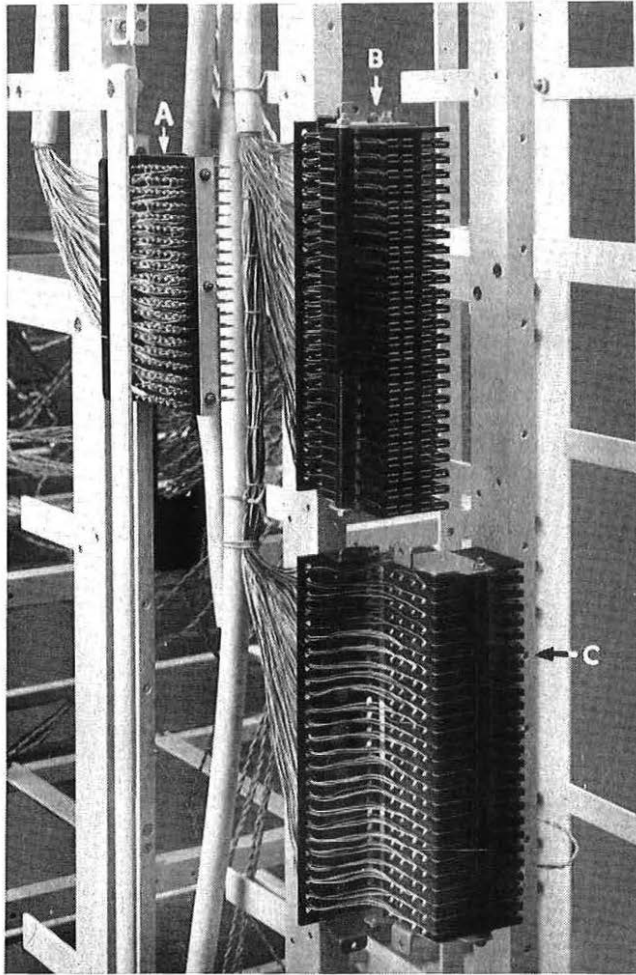
A—connexion strip; B—test-jack unit; C—test-jack unit swung outwards to facilitate access to permanent-wiring tags
