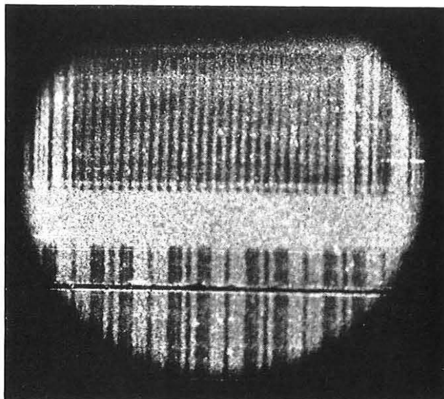
The recorded tracks are 0.030 in. wide and about 1,000 digits/inch can be recorded. The black line across the lower track is a joint between adjacent turns of tape; it is clear that joints do not interfere with the digits in any way. The digits have been made visible by the “Bitter figure” technique used for observing magnetic domains.
