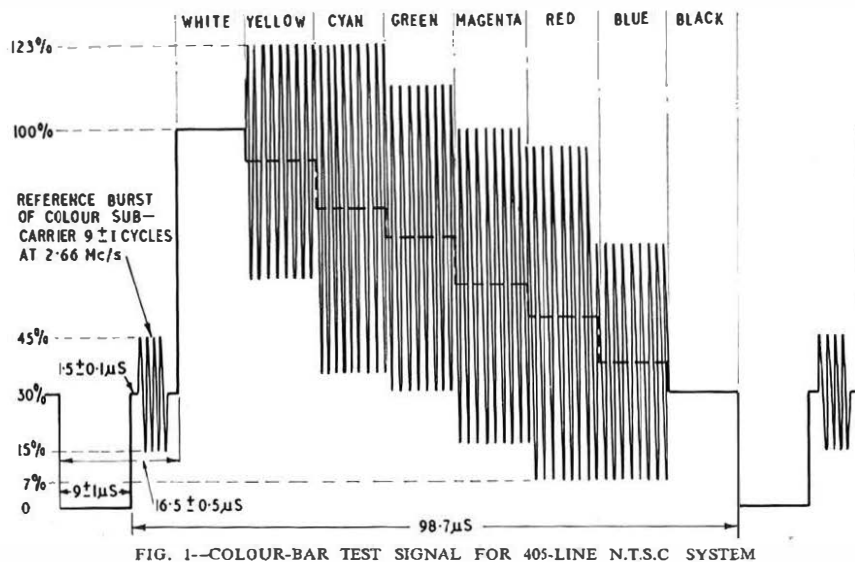
FIG. 1--COLOUR-BAR TEST SIGNAL FOR 405-LINE N.T.S.C. SYSTEM
