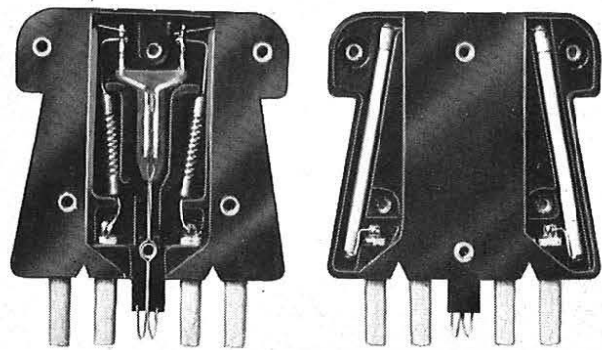
FIG. 6—WORKSOP TRIAL FUSE AND PROTECTOR PLUG
