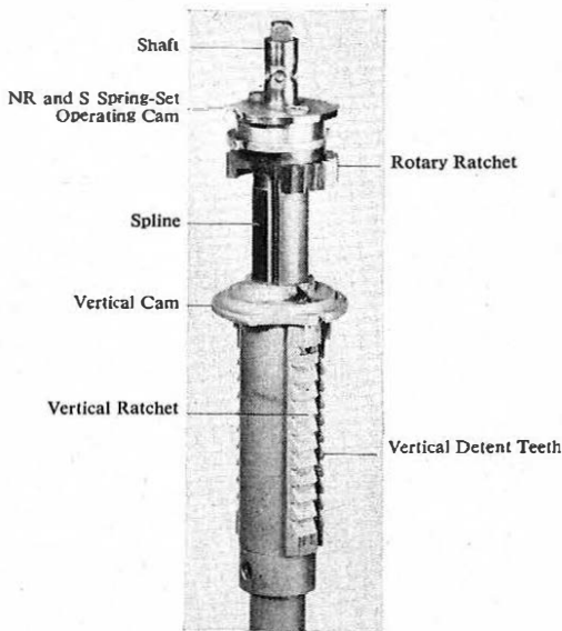
FIG. 3—RATCHET ASSEMBLY
