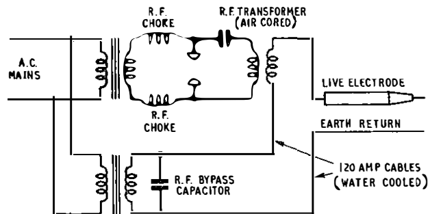
FIG. 25—ARGON-ARC WELDER
