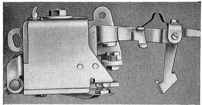
FIG. 4—VERTICAL-MAGNET ASSEMBLY
