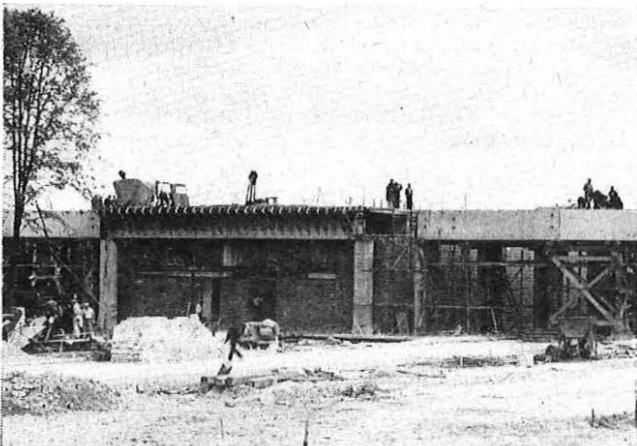
EARLY STAGE OF THE CONSTRUCTION OF THE NEW TERMINAL BUILDING, SHORTLY BEFORE THE INSTALLATION OF POST OFFICE EQUIPMENT
