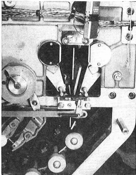
FIG. 8—DOUBLE WAITING-GATE
