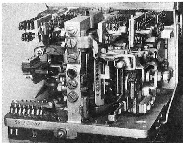
FIG. 7.—MECHANISM, SHOWING MECHANICALLY-OPERATED SPRING-SETS AND LINKAGES
