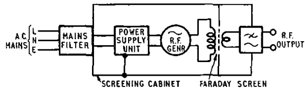
FIG. 24—MEDICAL DIATHERMY APPARATUS SHOWING INTERFERENCE-SUPPRESSION FEATURES
