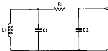
FIG. 9—DETAILS OF NETWORKS N_{SH} AND N_{SE}
