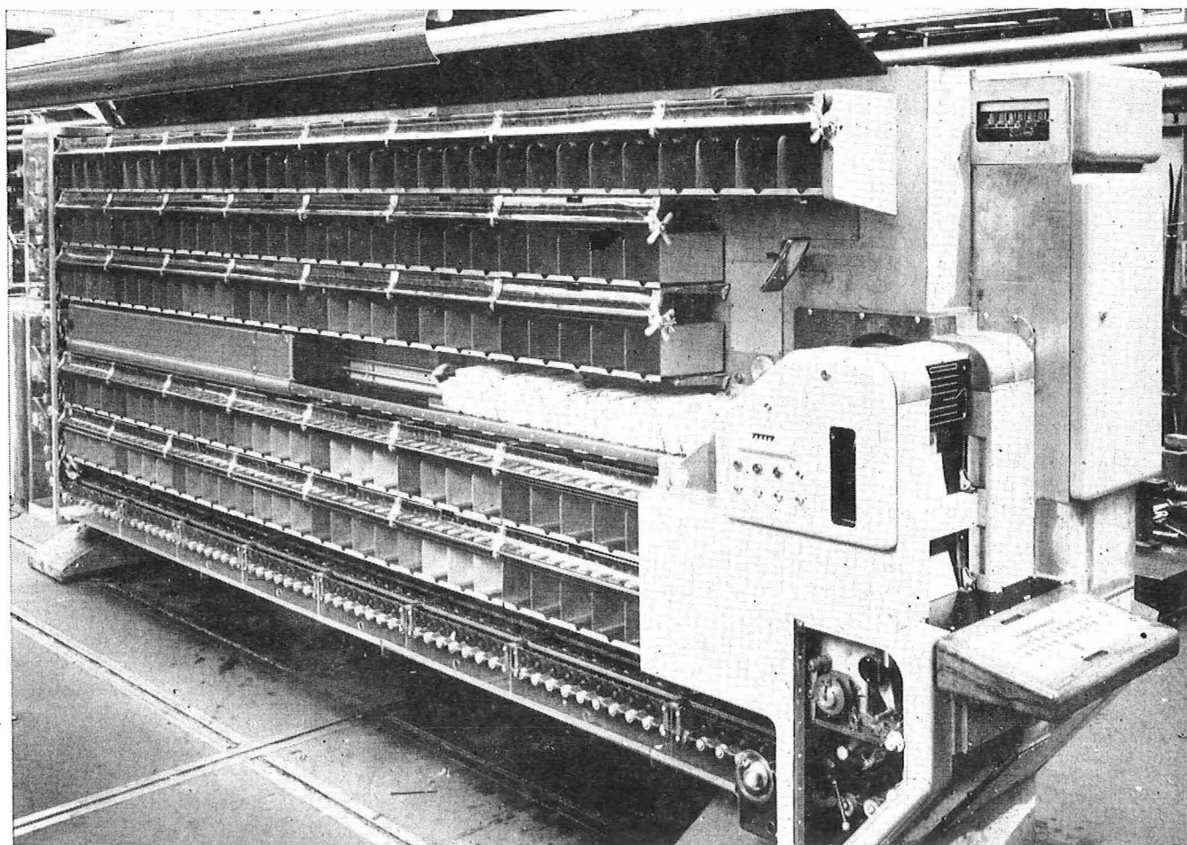
FIG. 5—THE PRODUCTION MACHINE
