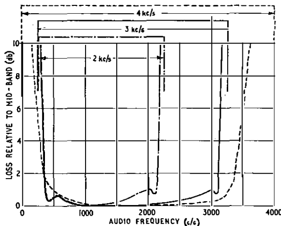
FIG. 3—TRANSMISSION-LOSS/FREQUENCY CHARACTERISTICS OF 2 KC/S, 3 KC/S AND 4 KC/S SPACED CARRIER CHANNELS
