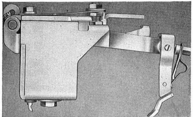
FIG. 5—ROTARY-MAGNET ASSEMBLY
