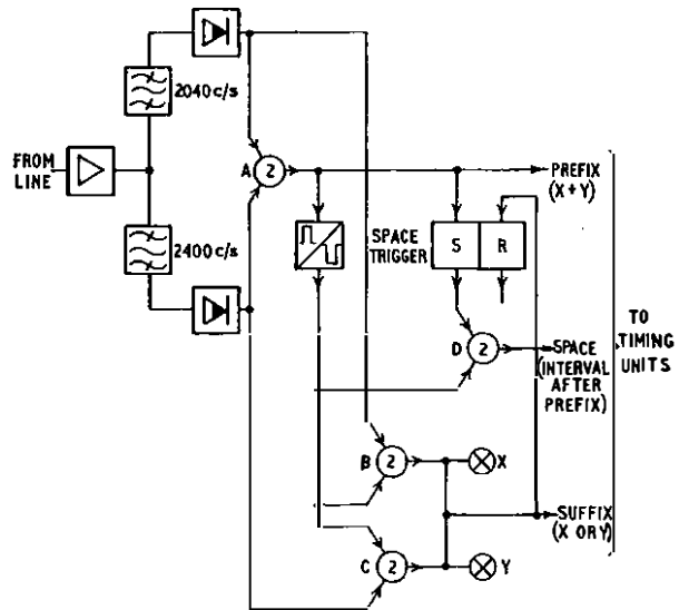
FIG. 3—THE 2 V.F. DETECTOR AND SEQUENCE CONTROL
