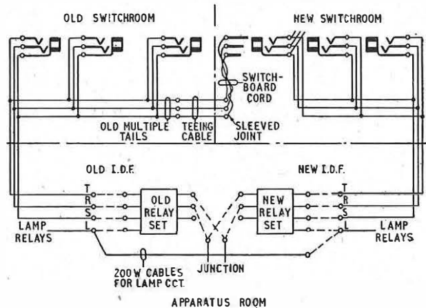
Connexions shown dotted to old relay-set were removed when those shown dotted to new relay-set had been provided
