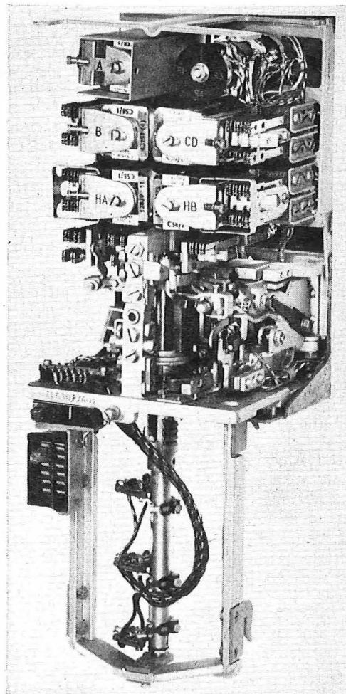
FIG. 1—THE 4000-TYPE GROUP SELECTOR
