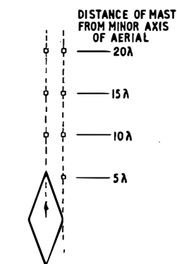
FIG. 12—POSITION OF MAST RELATIVE TO RHOMBIC AERIAL
