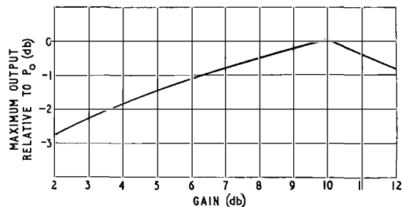
FIG. 10—EFFECT OF GAIN VARIATIONS ON MAXIMUM OUTPUT POWER FROM REPEATER
