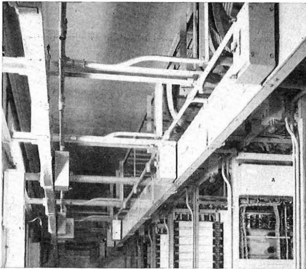
FIG. 4--POWER-DISTRIBUTION TRUNKING
