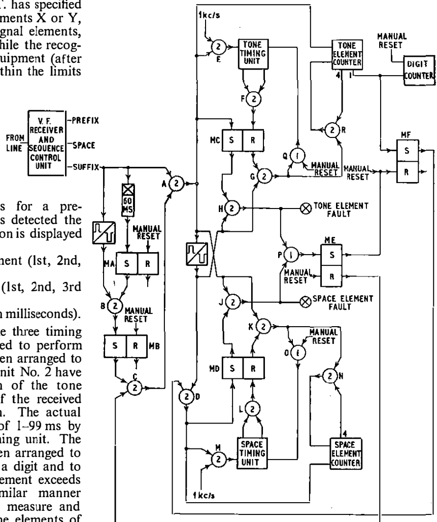
FIG. 5—LOGIC CIRCUIT FOR THE DIGIT CHECK
