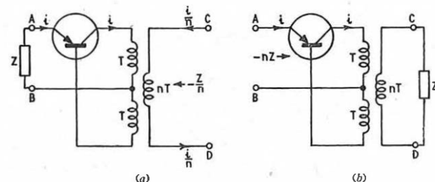
FIG. 4.—NEGATIVE-IMPEDANCE CONVERTOR
