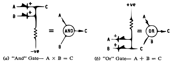
(a) “And” Gate— A \times B = C (b) “Or” Gate— A + B = C FIG. 7—TYPICAL DIODE GATES
