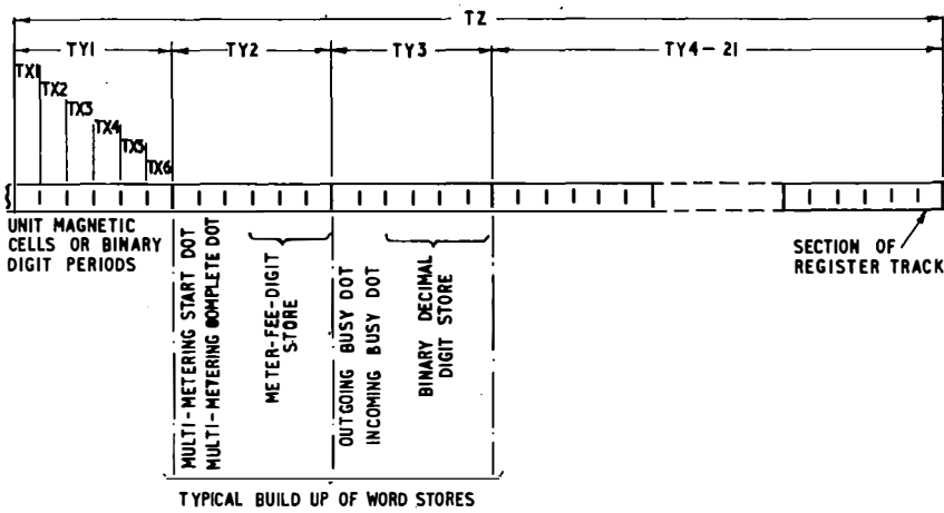
TYPICAL BUILD UP OF WORD STORES (a) Allocation of Timing Periods and Binary-Digit Cells
