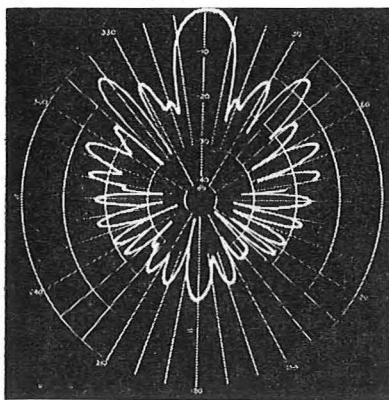
Photographed from face of cathode-ray tube FIG. 5—MEASURED DIRECTIVITY CHARACTERISTIC OF MODEL RHOMBIC AERIAL
