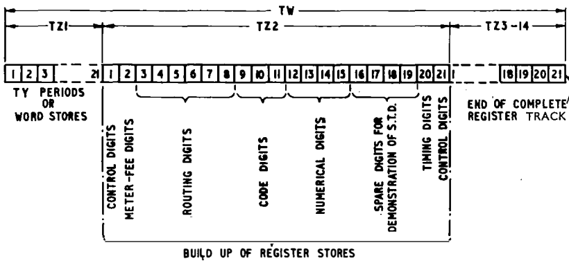
BUILD UP OF REGISTER STORES (b) Allocation of Timing Periods and Word Stores
