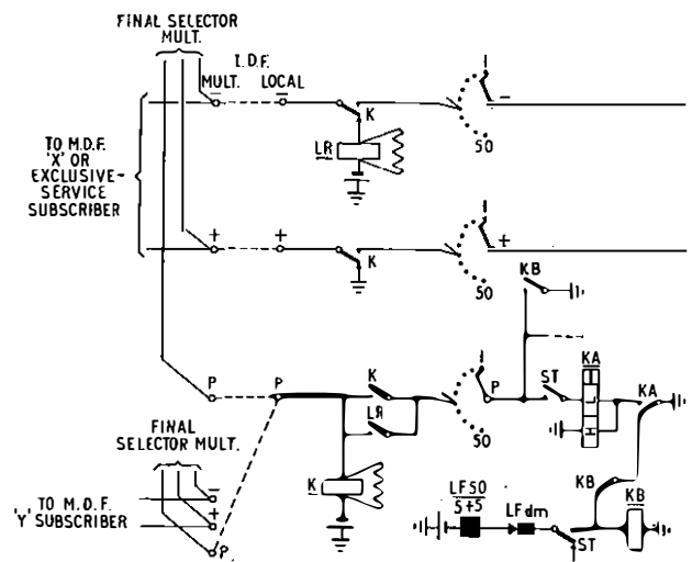
FIG. 7—SUBSCRIBER'S LINE CIRCUIT AND LINEFINDER SWITCHING CIRCUIT
