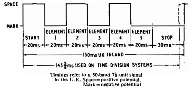
FIG. 1—EXAMPLE OF 5-UNIT CODE:—LETTER Y (MSMSM)
