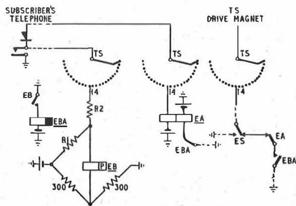
R1 = Signalling limit for exchange R2 = Half signalling limit for exchange FIG. 9—CALLING-EARTH AND RECTIFIER TEST
