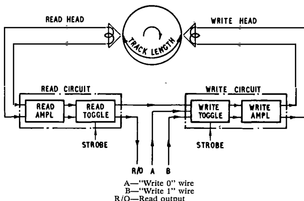
FIG. 4—REGENERATIVE-LOOP CIRCUIT FOR PHASE MODULATION RECORDING
