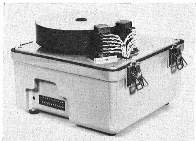
FIG. 2—MAGNETIC DRUM
