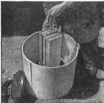
The repeater unit may be quickly removed from the buried repeater housing for inspection and maintenance.
