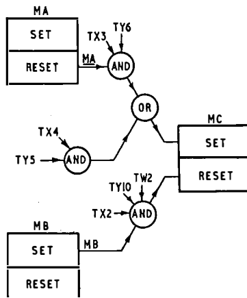
(b) \overline{MA} \times TX3 \times TY6 + TX4 \times TY5 = MC \overline{MB} \times TX2 \times TY10 \times TW2 = \overline{MC}
