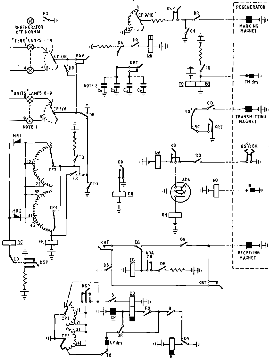
NOTE 1.—Units lamps multiplied at intervals of ten contacts NOTE 2.—Capacitors are strapped to give required pulse lengths
