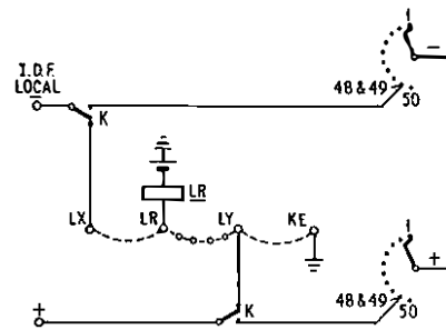
For normal service use connexions ----- To make X subscriber T.O.S. omit connexions ----- and use connexions - o - b - o - o - To make Y subscriber T.O.S. insulate contact of relay K which normally connects earth to line
