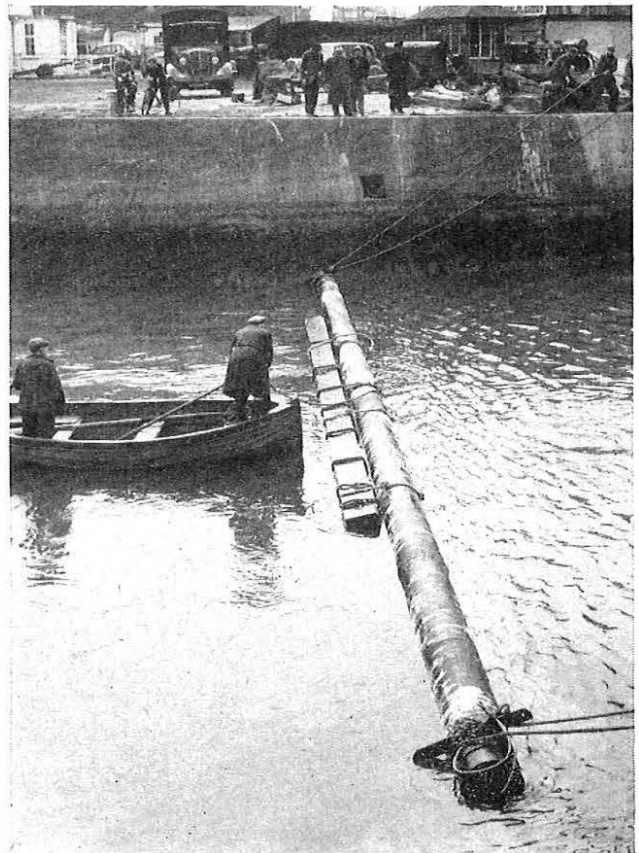
FIG. 10—MAIN-CROSSING PIPE BEING FLOATED INTO POSITION
