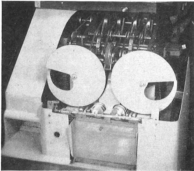
The four helices, two large and two small, can be seen at the front. FIG. 3—LETTER-PRESENTATION SECTION WITH COVER REMOVED
