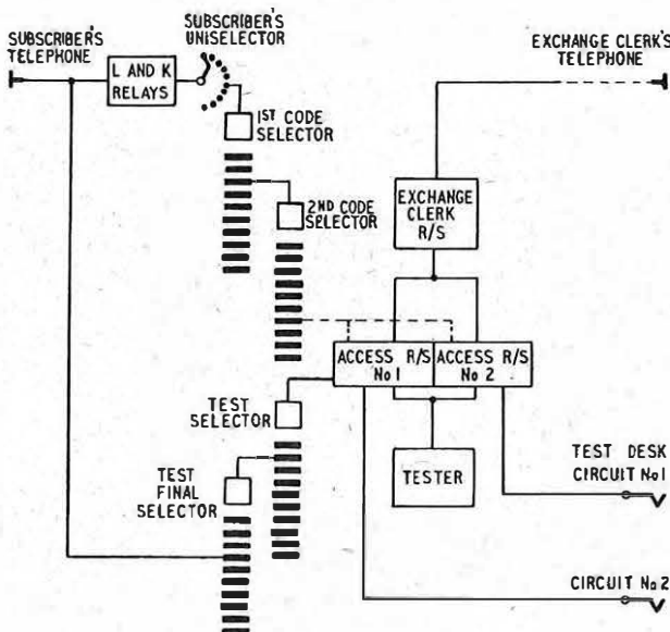
FIG. 1—TRUNKING OF MODEL 2 SUBSCRIBER'S LINE TESTER
