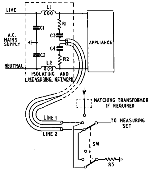
Up to 30 Mc/s: R_1 = R_2 = 75 \text{ ohms} ; R_3 = 150 \text{ ohms} Above 30 Mc/s: R_1 = R_2 = 0 \text{ ohms} ; R_3 = 75 \text{ ohms} FIG. 18—ARRANGEMENT FOR MAINS-VOLTAGE AND FIELD-STRENGTH MEASUREMENTS
