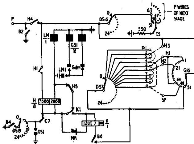
FIG. 6.—HUNTING, TESTING AND SWITCHING CIRCUIT.
