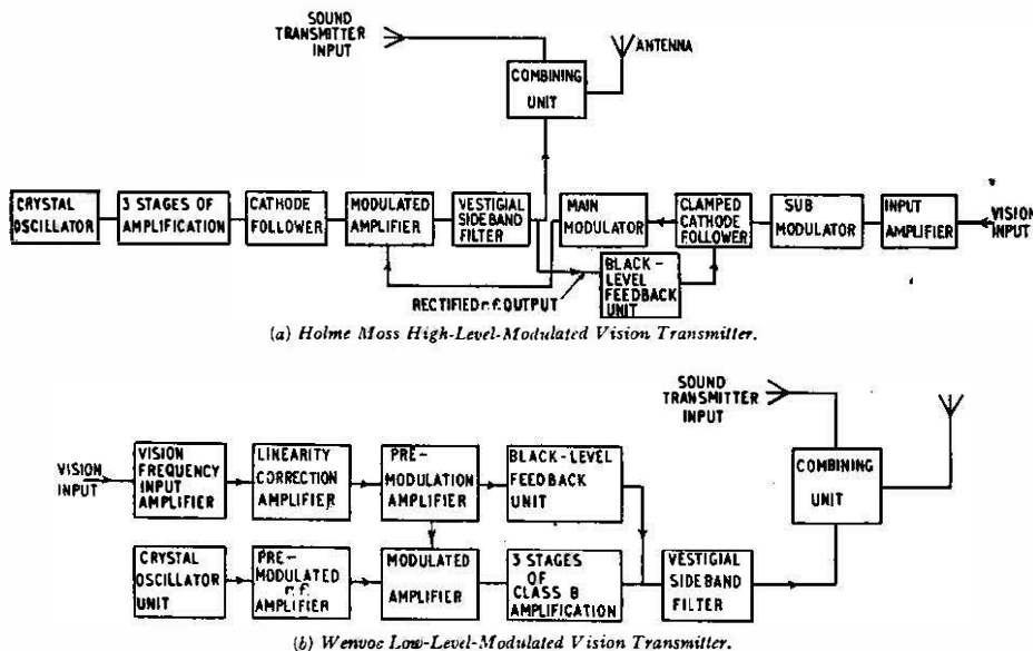
FIG. 5.—BLOCK SCHEMATIC DIAGRAMS OF TWO MODERN VISION TRANSMITTERS.
