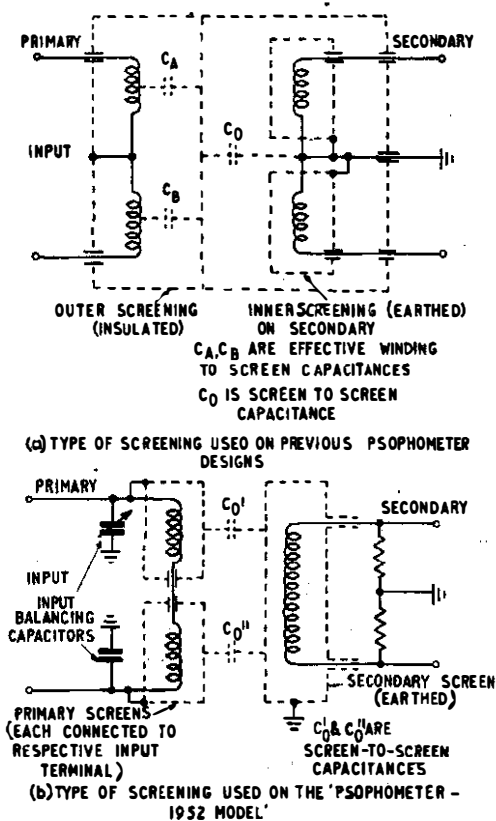
FIG. 4.—METHODS OF SCREENING INPUT TRANSFORMERS.
