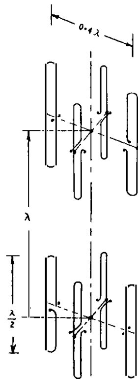
FIG. 6.—FOLDED-DIPOLE TYPE TRANSMITTING ANTENNA.
