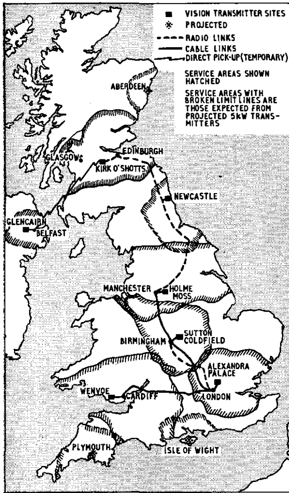
FIG. 2.—THE BRITISH TELEVISION NETWORK.
