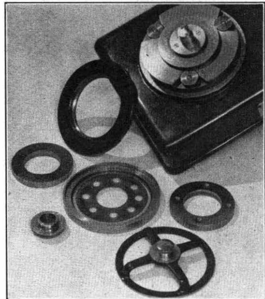
FIG. 3.—COMPONENTS OF THE NEW MACHINE.
