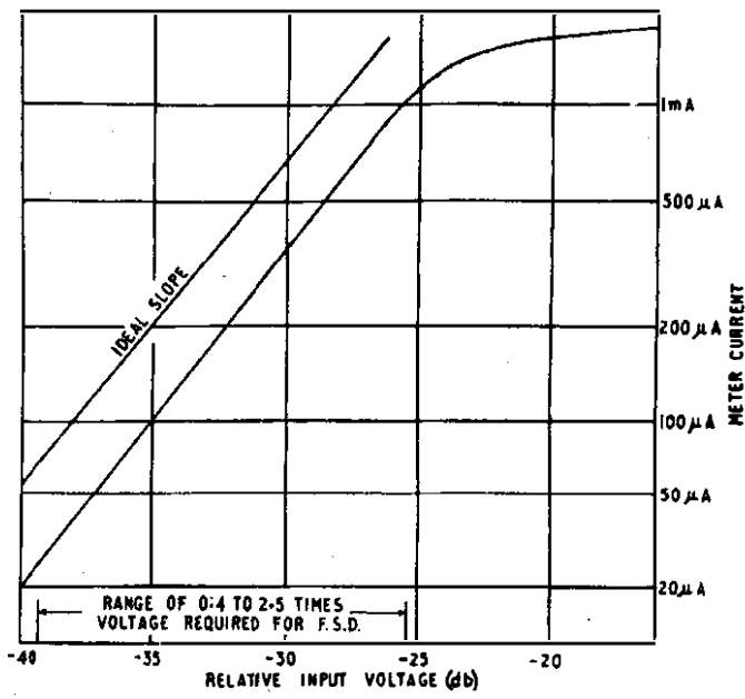
FIG. 7.—INPUT VOLTAGE/METER CURRENT CHARACTERISTIC OF SQUARE-LAW CIRCUIT FOR SINGLE FREQUENCY (1 KC/S) INPUT.
