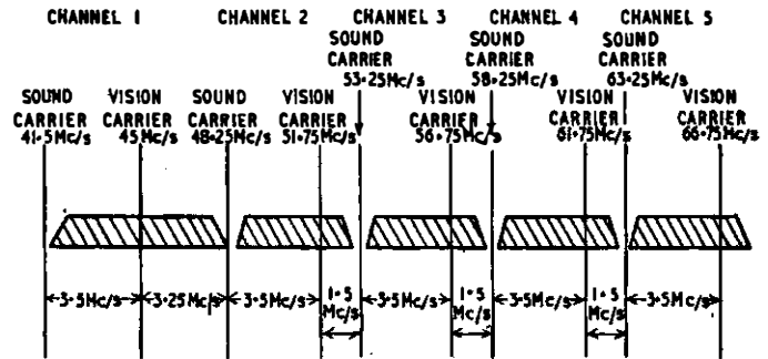
FIG. 1.—FREQUENCIES ALLOCATED TO BRITISH TELEVISION CHANNELS.
