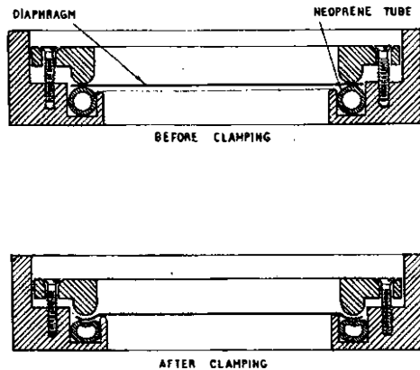
FIG. 5.—A TENSIONING FRAME FOR DIAPHRAGM OF LAPPING MACHINE.
