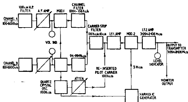
FIG. 3.—ARRANGEMENT OF TRANSMITTER-DRIVE UNIT.
