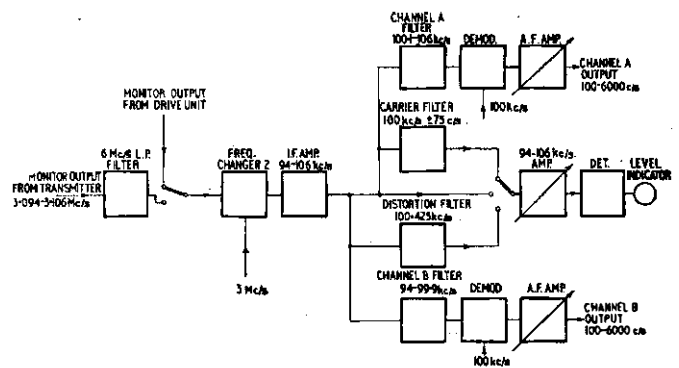
FIG. 5.—BLOCK SCHEMATIC DIAGRAM OF MONITORING EQUIPMENT.
