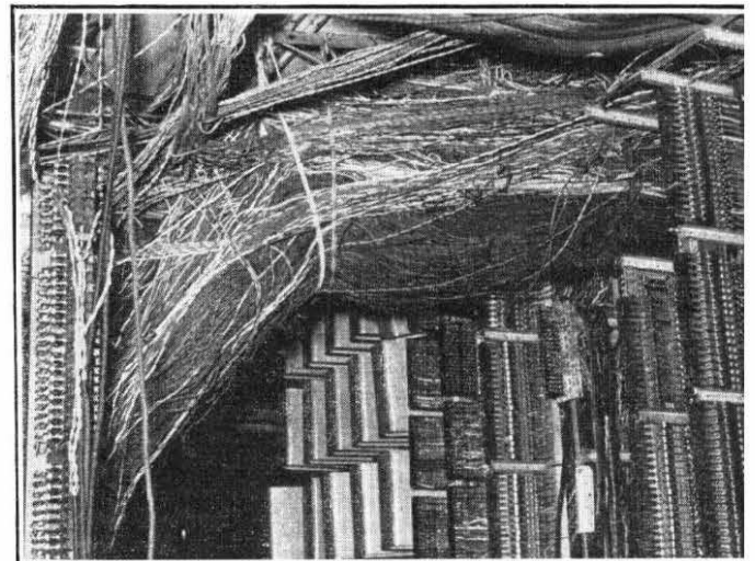
M.D.F. WIRING IN CARDIFF MANUAL EXCHANGE.
