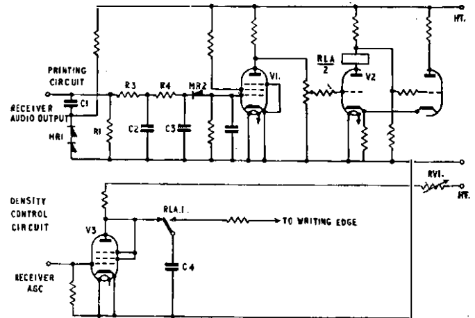
FIG. 5.—CIRCUIT DIAGRAM OF RECORDER.
