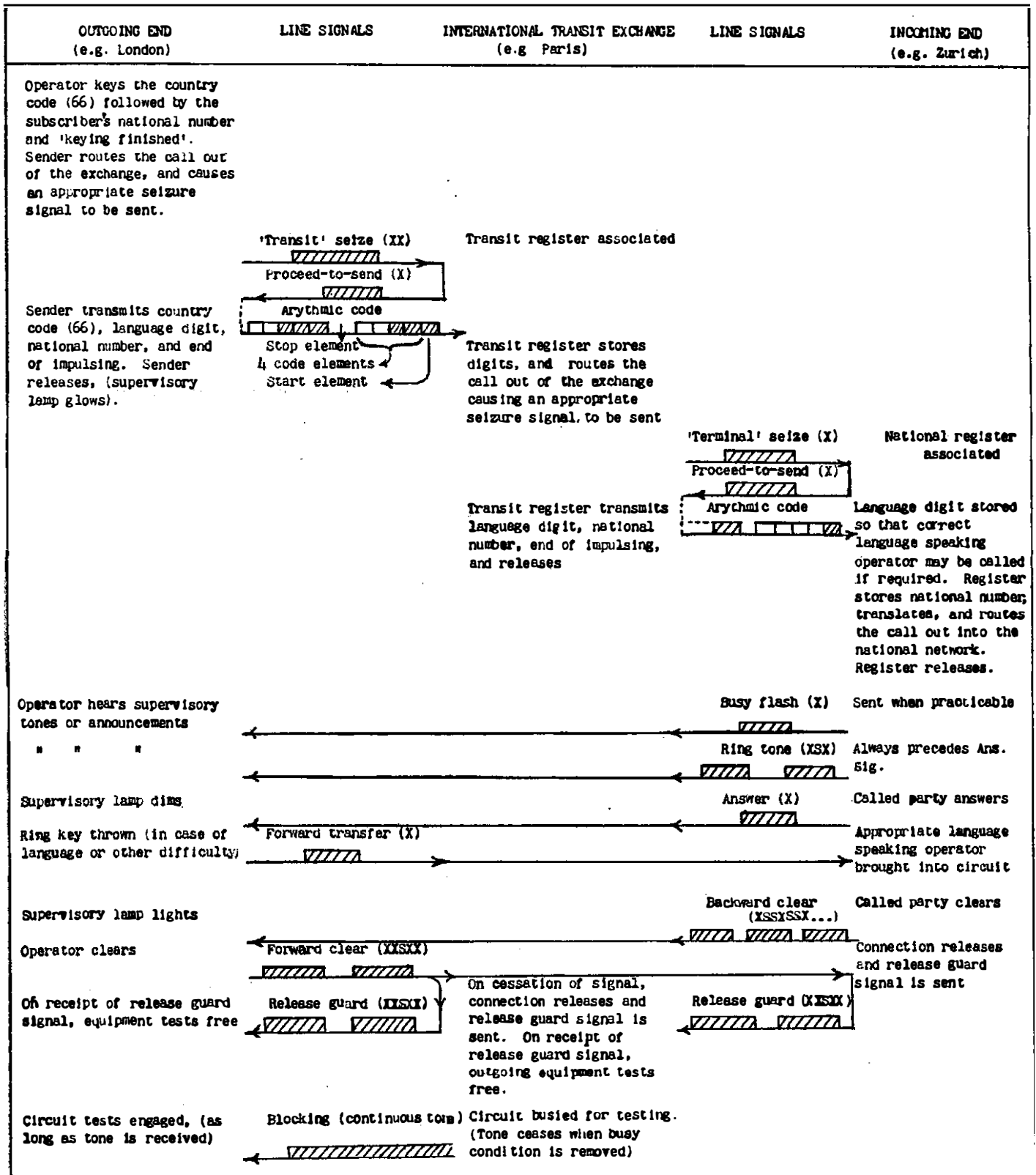
FIG. 5.—APPLICATION OF THE SIGNAL CODE—I V.F. SYSTEM.
