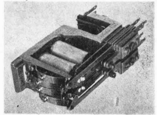
TYPE 100 HIGH-SPEED RELAY with double changeover action.
