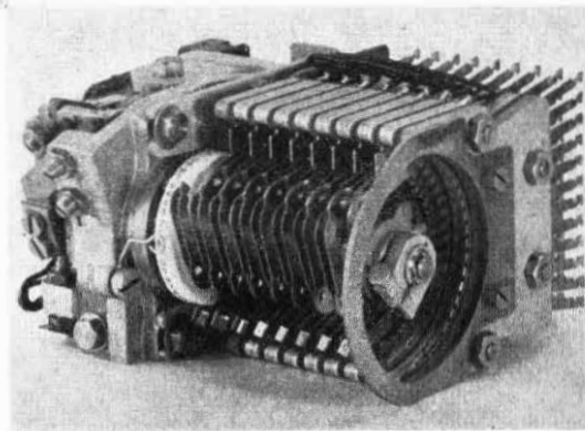
MOTOR UNISELECTOR operates at 200 steps per second.
