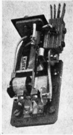
TYPE 89 HIGH-SPEED RELAY with single changeover.
