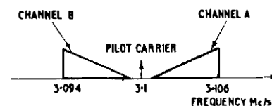
FIG. 2.—INDEPENDENT-SIDE-BAND SIGNAL PRODUCED BY DRIVE EQUIPMENT.
