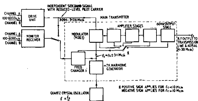
FIG. 1.—RELATIONSHIP OF DRIVE EQUIPMENT AND MONITOR RECEIVER TO MAIN TRANSMITTER.
