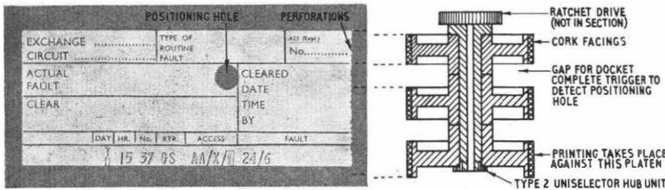
FIG. 2.—COMPLETED DOCKET AND PLATEN IN SECTION.
