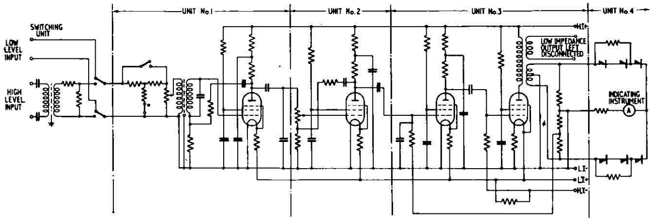
FIG. 4.—CIRCUIT OF A.C. VOLTMETER AND AMPLIFIER.
