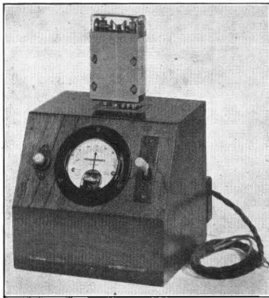
FIG. 1.—TESTER WITH RELAY IN POSITION.
