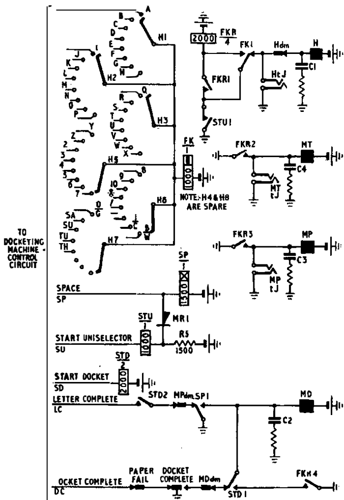
FIG. 7.—CIRCUIT OF RECORDER.
