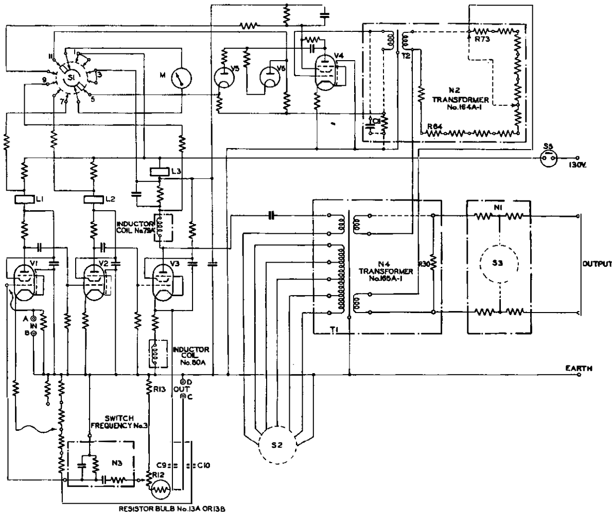
FIG. 5.—SIMPLIFIED CIRCUIT DIAGRAM OF OSCILLATOR NO. 22.
