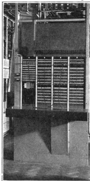
FIG. 2.—THE ENGINEERING CONTROL BOARD.
