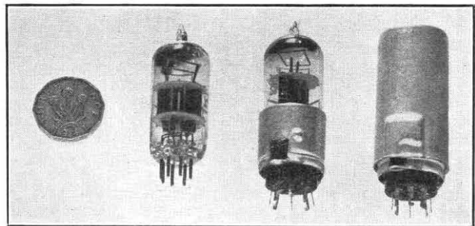
FIG. 6.—HOT-CATHODE VALVE OF B7G TYPE.
