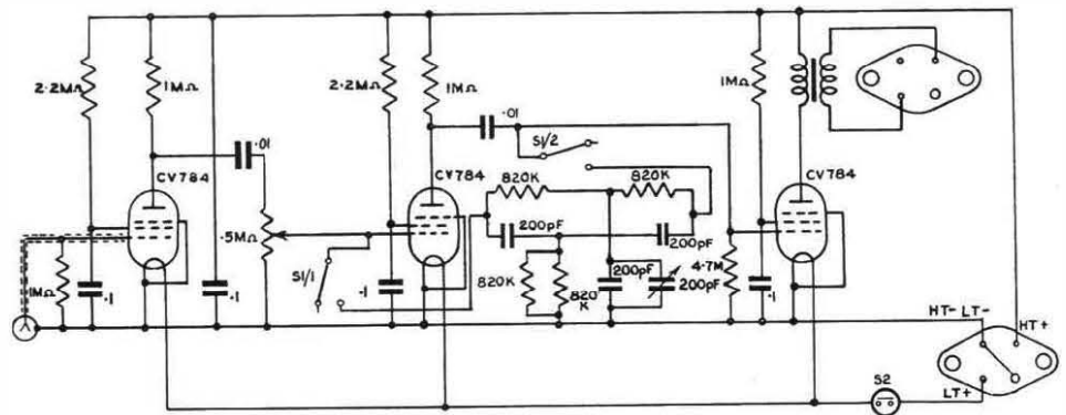
FIG. 5.—CIRCUIT DIAGRAM OF THE AMPLIFIER.
