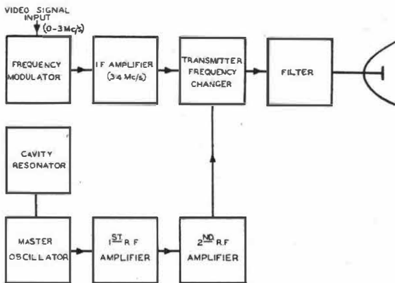
FIG. 8.—BLOCK SCHEMATIC OF TERMINAL TRANSMITTER.
