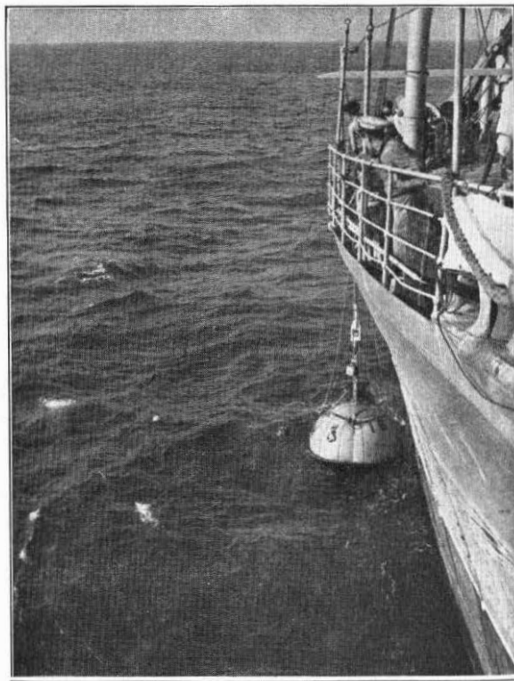
FIG. 3.—VIEW, LOOKING AFT, OF BUOY COMING IN ALONGSIDE SHIP AND SEAMEN HOOKING "TAIL" WITH GRAPNELS.
