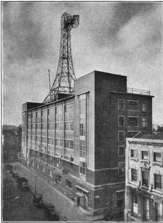
FIG. 7.—THE TOWER AT MUSEUM EXCHANGE, LONDON.
