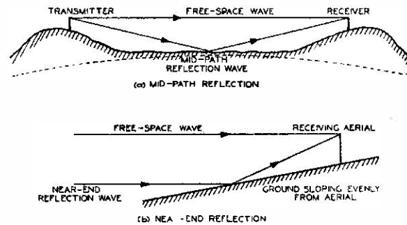
FIG. 2.—PROPAGATION OF FREE-SPACE AND REFLECTED WAVES.
