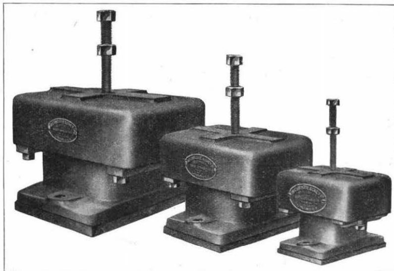
FIG. 5.—PEDESTAL-TYPE ANTI-VIBRATORS.
