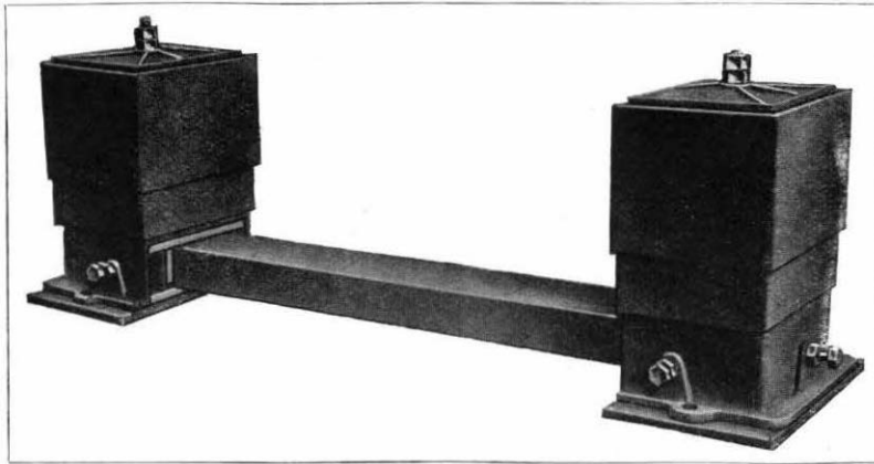
FIG. 6.—BRIDGE-TYPE ANTI-VIBRATOR.
