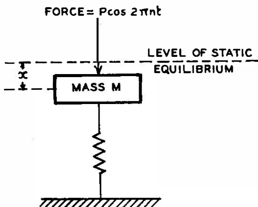
FIG. 3.—FORCED VIBRATION OF A MASS SUPPORTED ON A SPRING.
