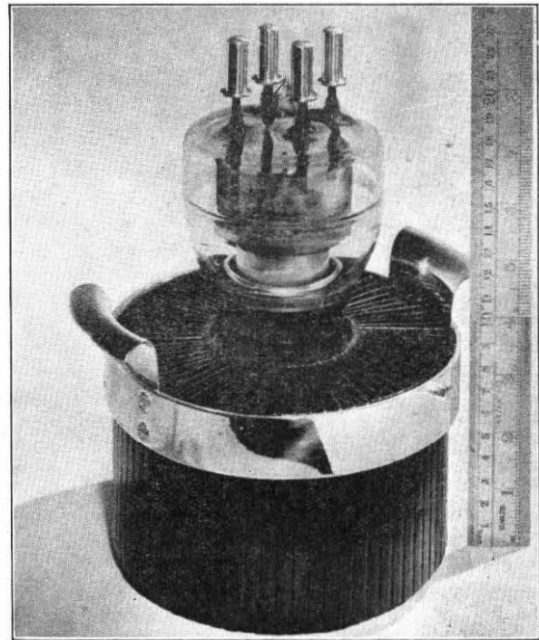
FIG. 6.—FORCED-AIR-COOLED TRIODE, 4.5 KW ANODE DISSIPATION.
