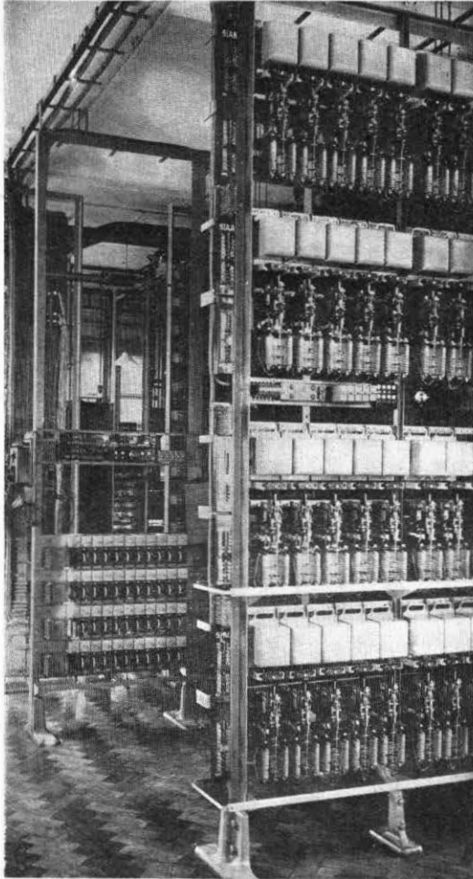
Automatic hooks Preston Exchange, Brighton (1927)
