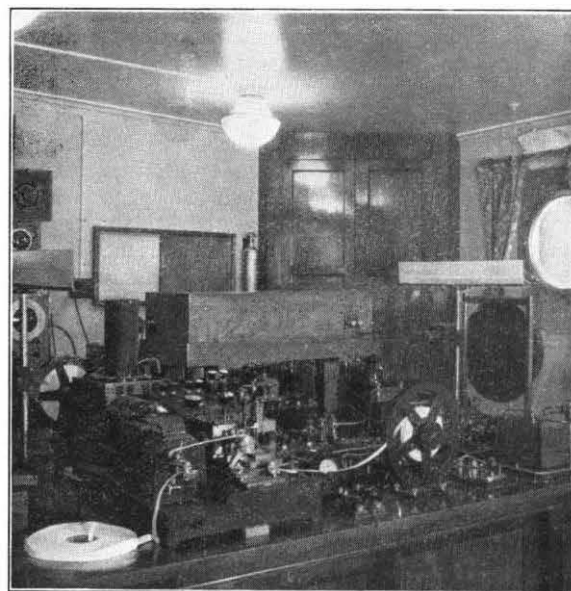
FIG. 2.—THE MAIN TEST TABLE, SHOWING SYPHON RECORDER AND D.R. TEST SET.
