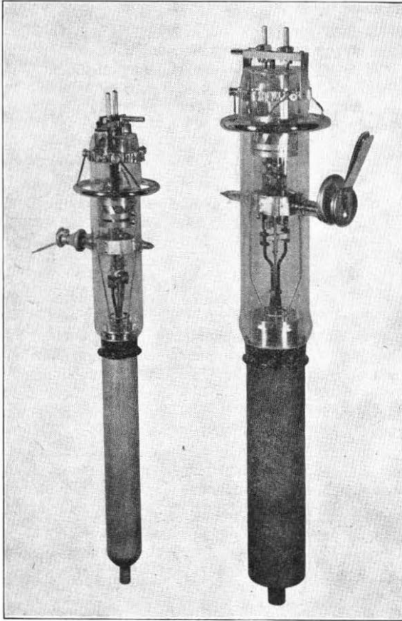
FIG. 5.—18-KW TRIODE (RIGHT) AND 12-KW TRIODE, WITH SIDE-ENTRY GRID SEALS.
