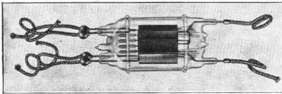
FIG. 1.—1.5-kW SILICA ENVELOPE VALVE.
