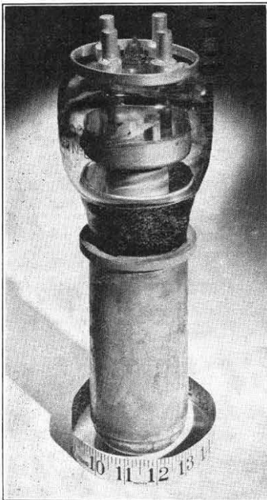
FIG. 3.—SINGLE-ENDED 20-KW WATER-COOLED TRIODE WITH THORIATED-TUNGSTEN FILAMENT.
