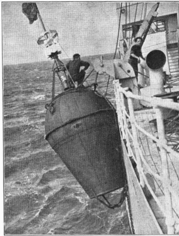
FIG. 5.—BUOY HOISTED TO DECK LEVEL ON SPECIAL SHEAVE.
