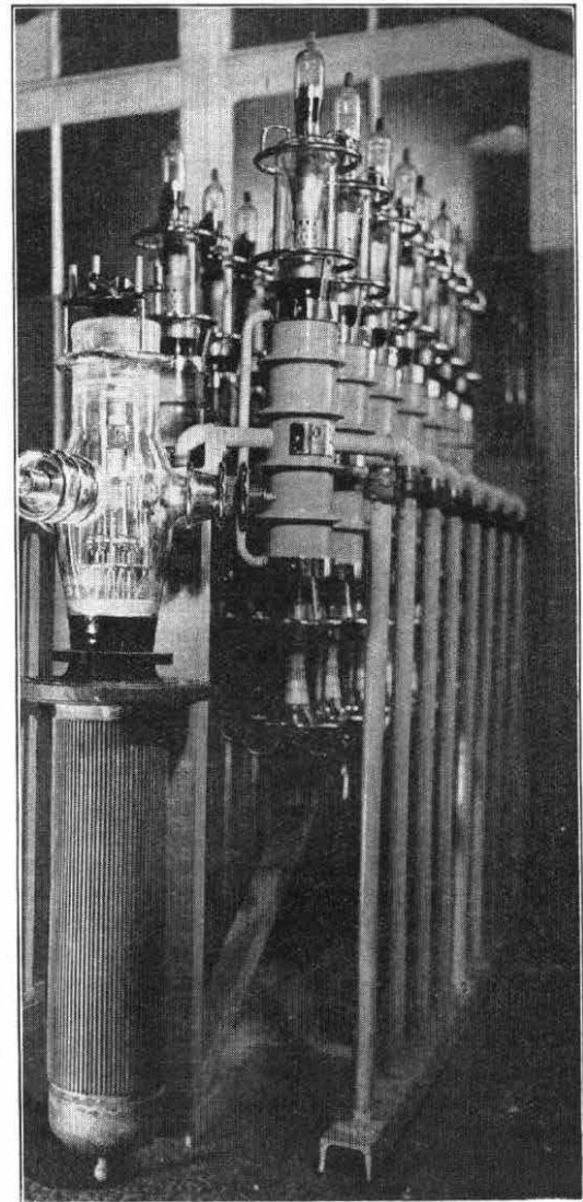
FIG. 2.—160-kW WATER-COOLED TRIODE AND A BANK OF 80-kW DOUBLE-ENDED WATER-COOLED TRIODES.
