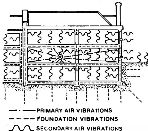
FIG. 1.—VIBRATIONS TRANSMITTED BY A MACHINE NOT ISOLATED FROM ITS BED.
